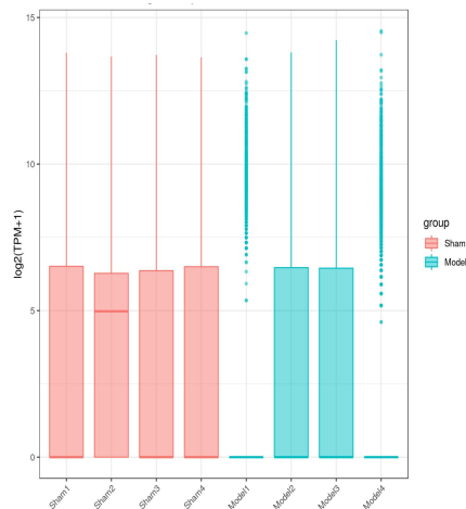
A Gene Expression Distribution
