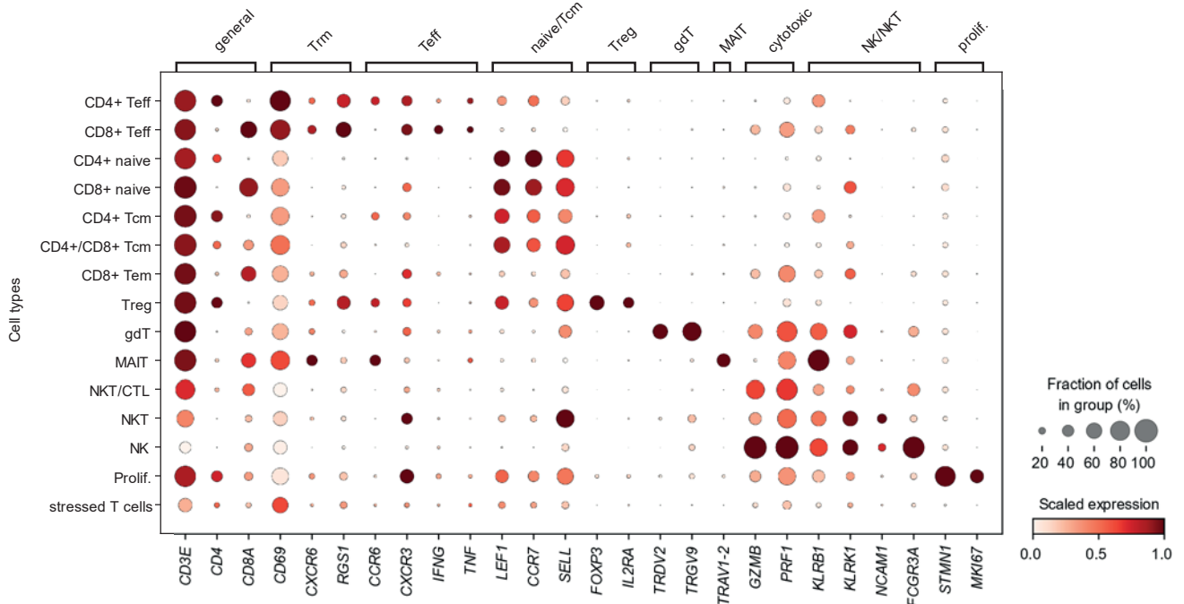
Supplemental Figure 2: Exploratory cohort single cell T cell atlas. a Quality control metrics and tissue composition across patients and cell type clusters. Violin plots show distributions of the number of genes, total counts, percentage of mitochondrial counts, and percentage of ribosomal counts. Barplots visualize the relative tissue composition and the total number of cells on a log scale. b Marker gene expression for the broad T cell annotations.
