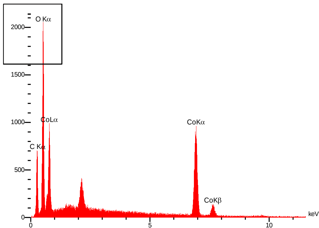
Figure 1S. EDS Analysis of the RGOCoo hybrid.
