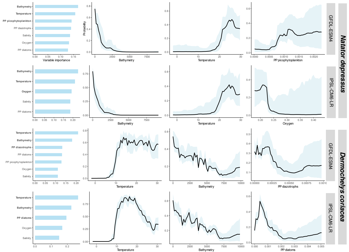
Figure 3. Contributions of all the variables to the model for both ESMs are presented. We also provide the additive relation for the variables that have contributed the most to the model. These additive relations represent the probability of being present at some point along the x-axis.
