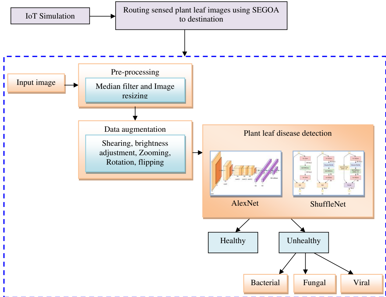
Figure 2: Architectural representation of proposed methodology
