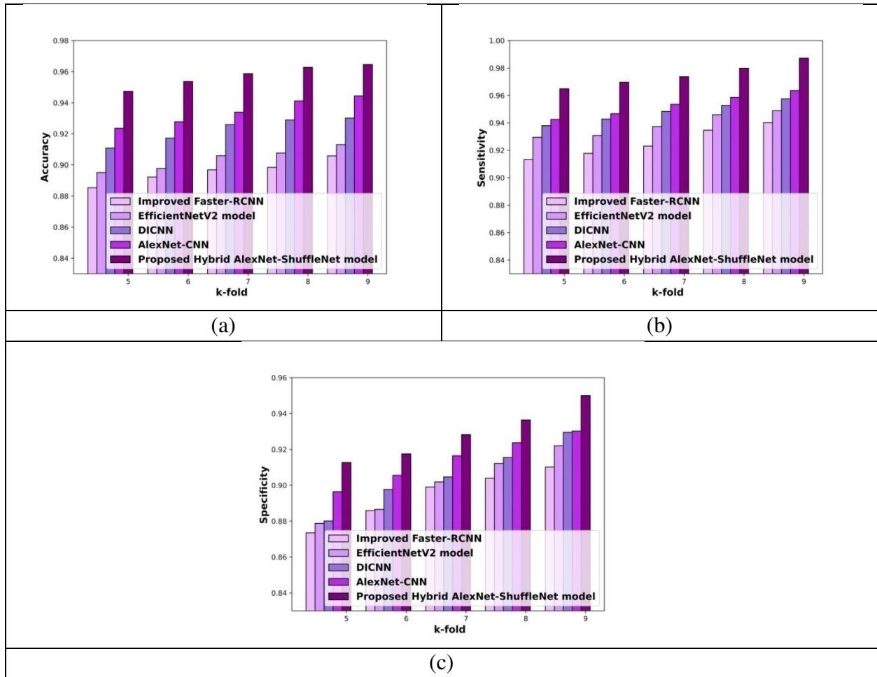
Figure 7: Comparative measurement of techniques with k fold (a) accuracy (b) sensitivity (c) specificity
