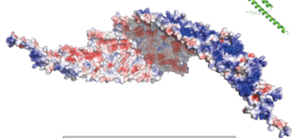
StREM1.3/67-198 12-Mers
