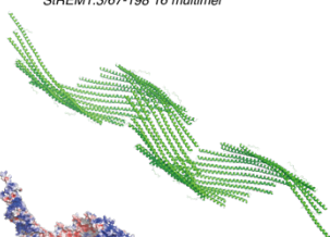
StREM1.3/67-198 16 multimer
