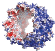
StREM1.3/67-198 16 multimer
