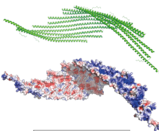
StREM1.3/67-198 12-Mers
