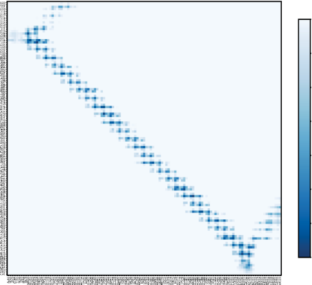
AtREM6.6/233-345_Dimer_All-Atom
