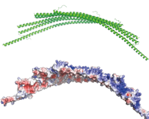
StREM1.3/67-198 12-Mers
