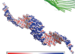
StREM1.3/67-198 32 multimer
