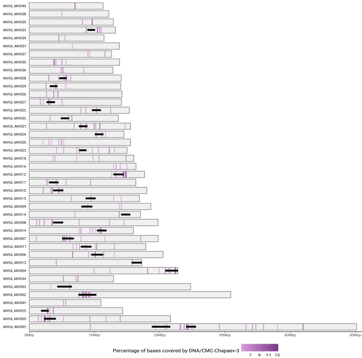
Supplementary Data 7. CMC-Chapaev3 transposable elements in other earthworms ( Metaphire vulgaris , MVUL, and Carpetania matritensis , CMAT), showing their overall overlap with centromeres (black lines).
