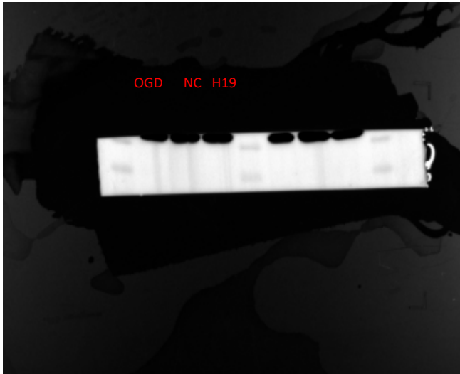
\beta -actin
