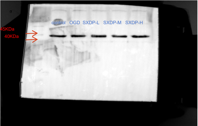
\beta -actin
