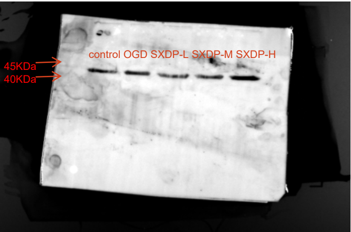
\beta -actin
