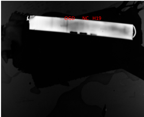
P66 shc
