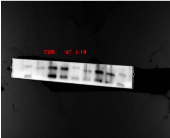
P-P66 shc
