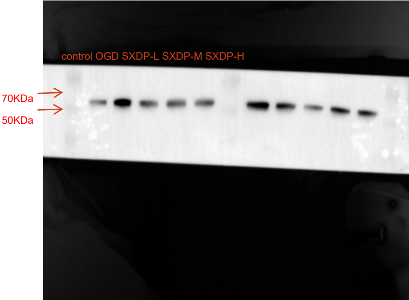
P66 shc
