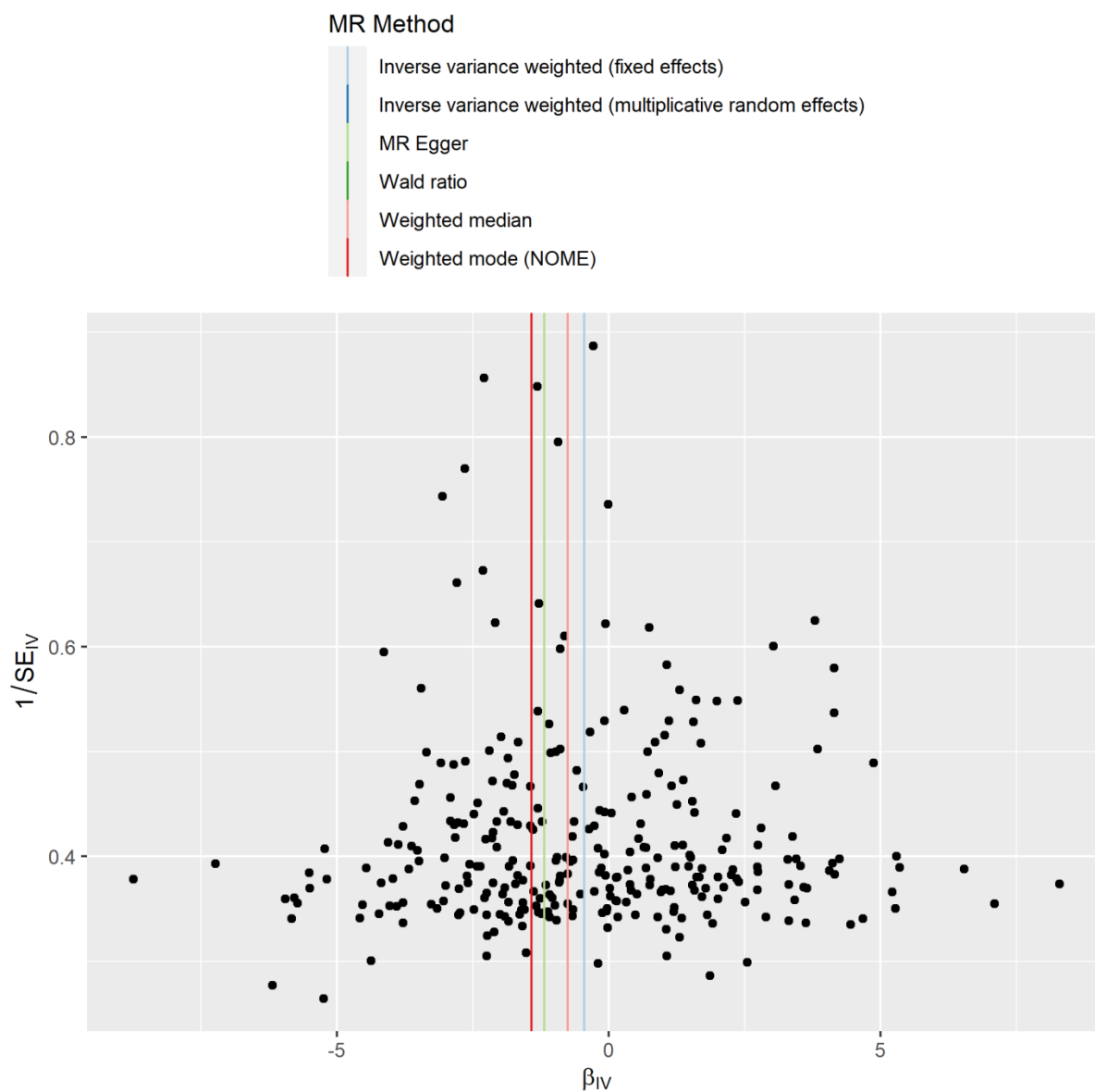
Fig.S22 Funnel plot of SNPs associated with education and their risk of ER- (GWAS)
