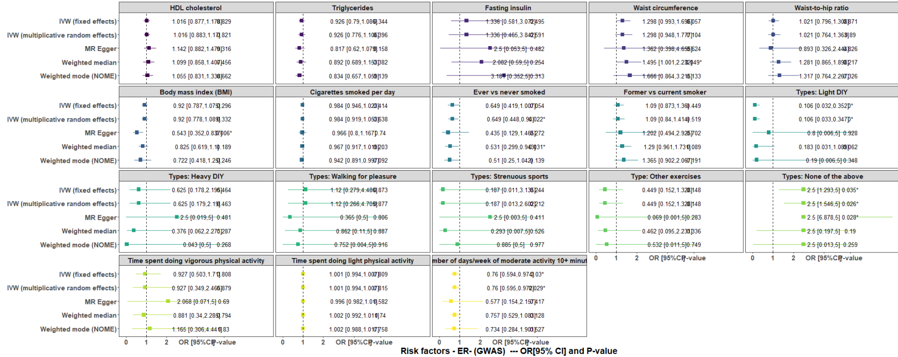
Fig.S4 Causal estimates of potential mediators on ER- (GWAS)
