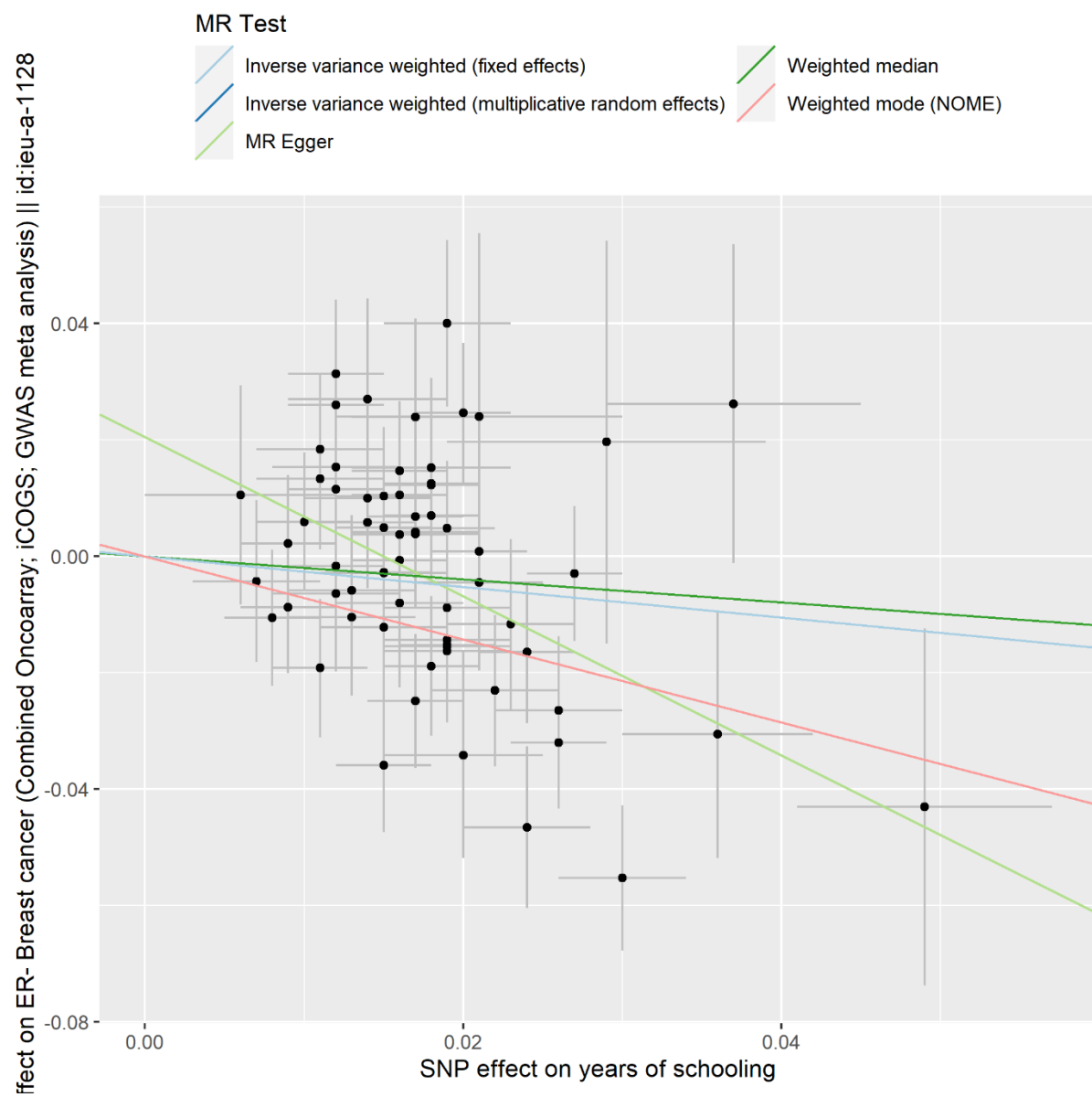
Fig.S8 Scatter plot of SNPs associated with education and their risk of ER- (combined)
