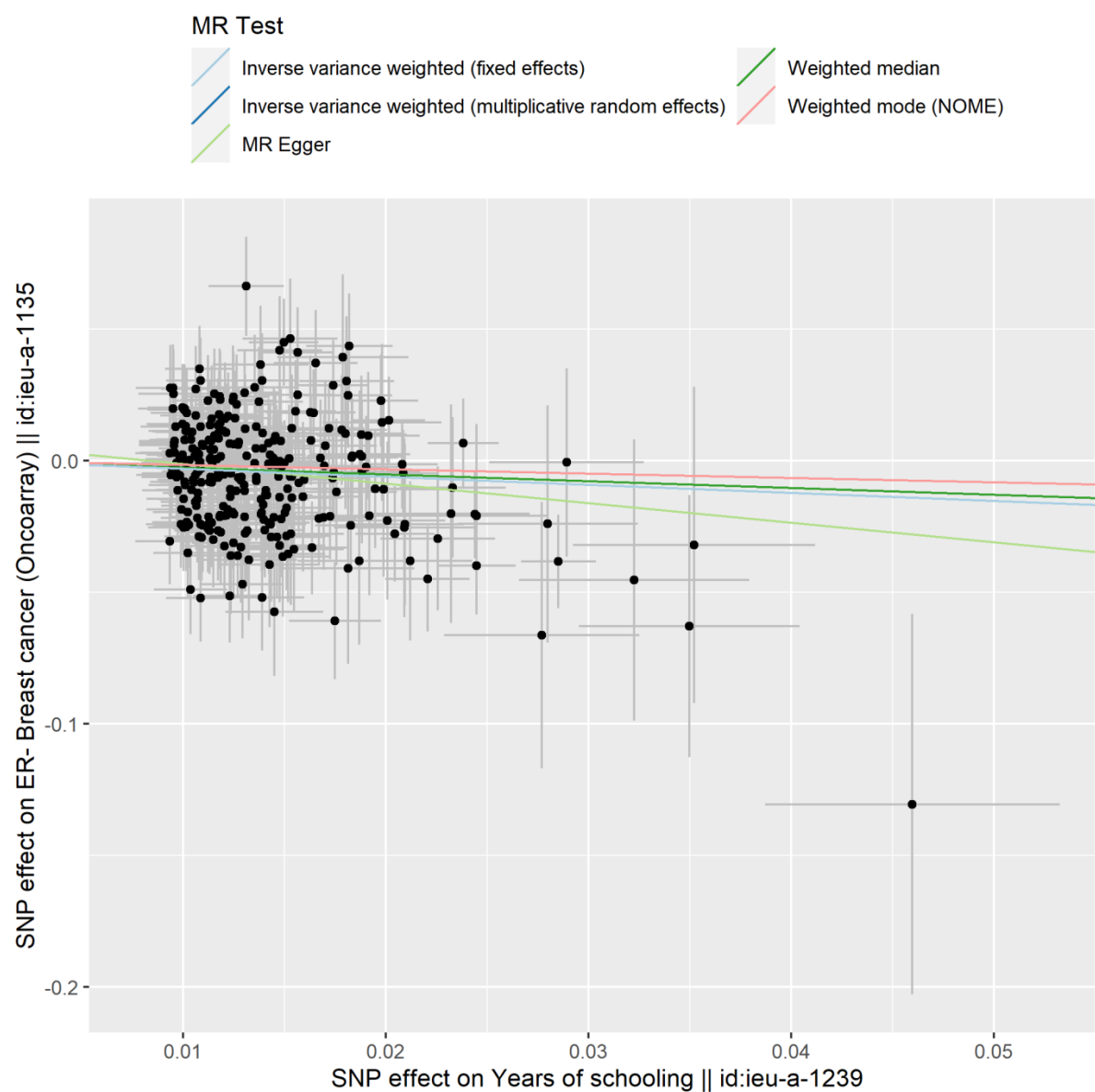
Fig.S12 Scatter plot of SNPs associated with education and their risk of ER- (Oncoarray)
