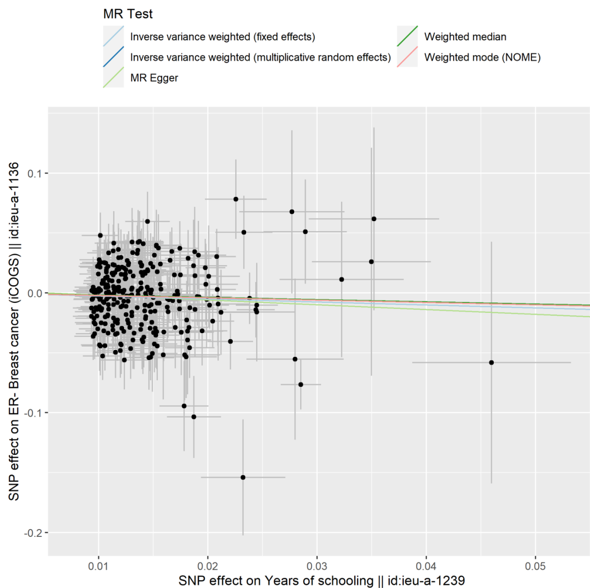
Fig.S16 Scatter plot of SNPs associated with education and their risk of ER- (iCOGS)
