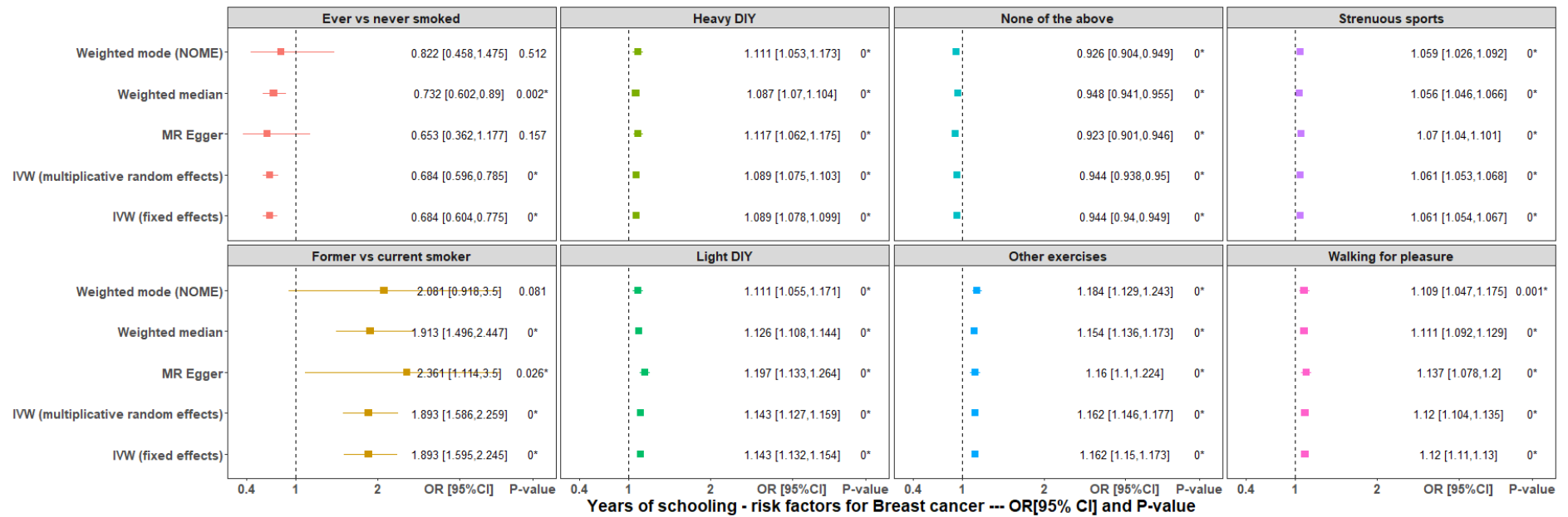
Fig.S1 Causal estimates of education on potential mediators (binary)
