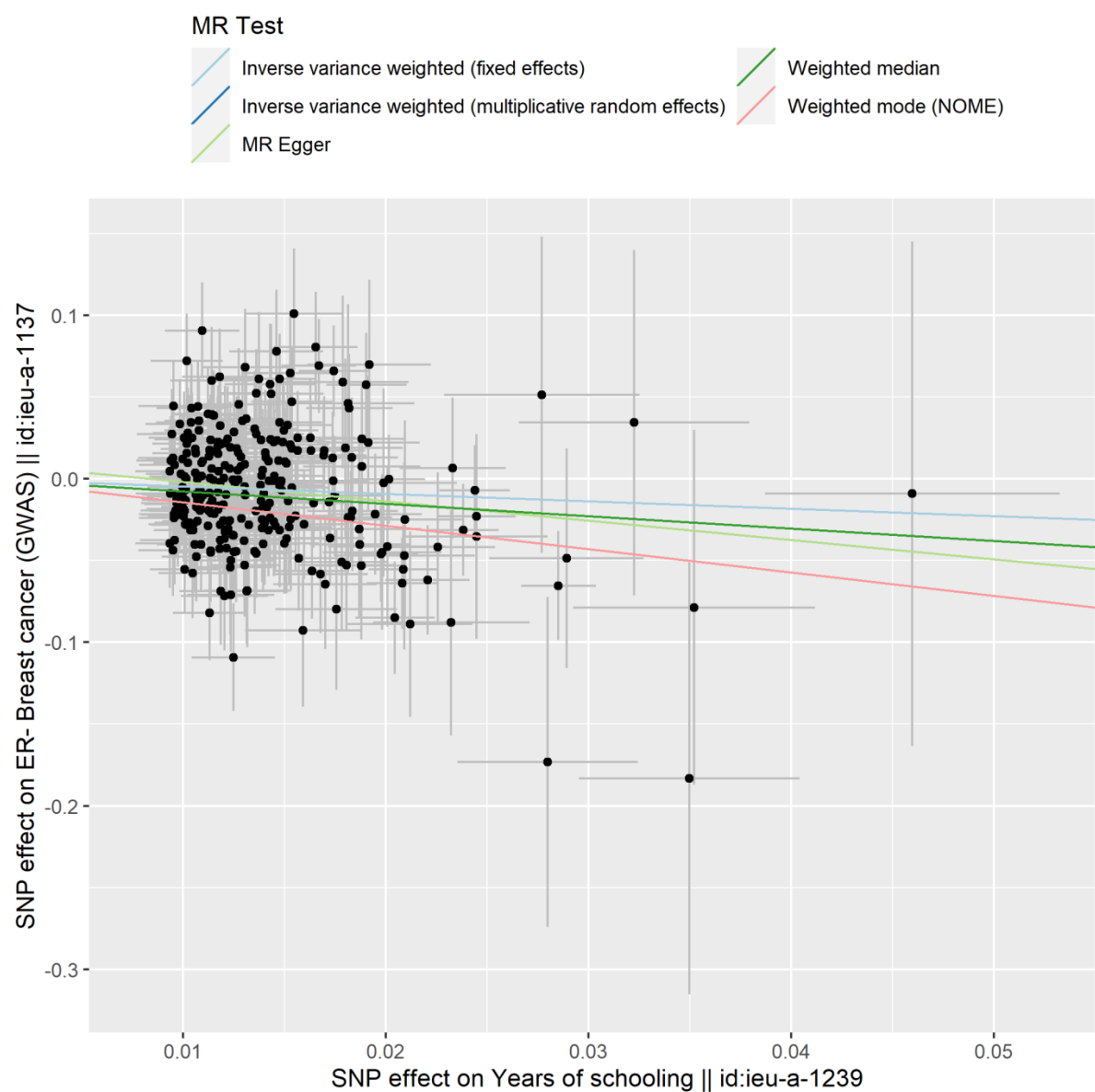
Fig.S20 Scatter plot of SNPs associated with education and their risk of ER- (GWAS)
