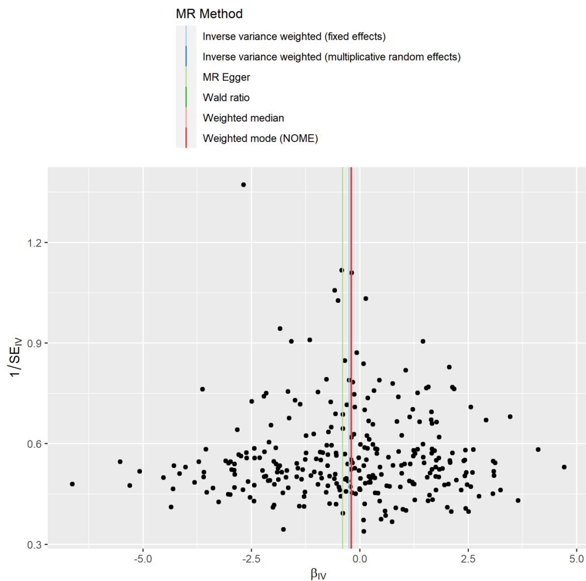
Fig.S18 Funnel plot of SNPs associated with education and their risk of ER- (iCOGS)
