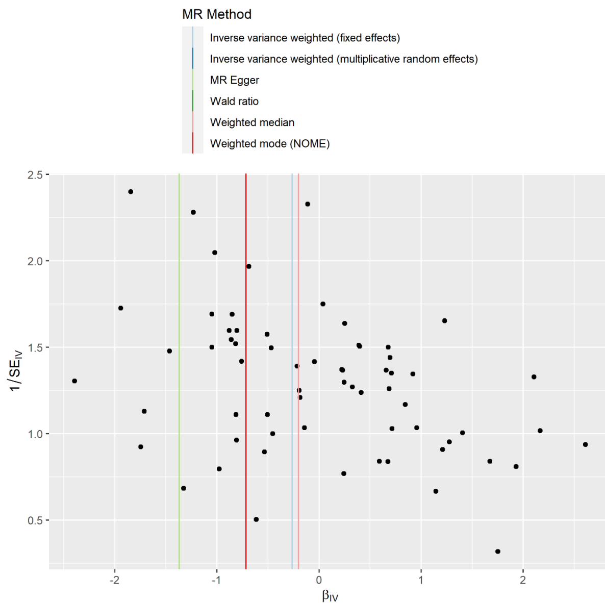
Fig.S10 Funnel plot of SNPs associated with education and their risk of ER- (combined)
