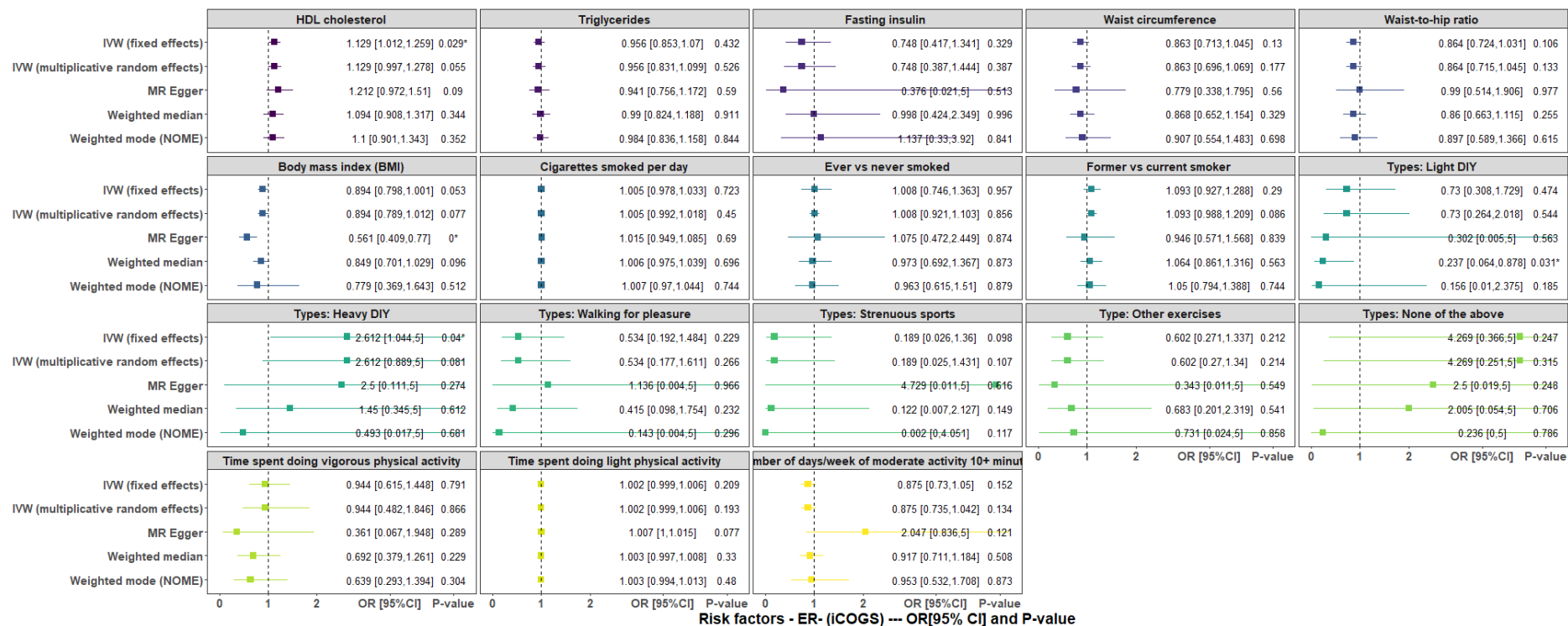
Fig.S5 Causal estimates of potential mediators on ER- (iCOGS)
