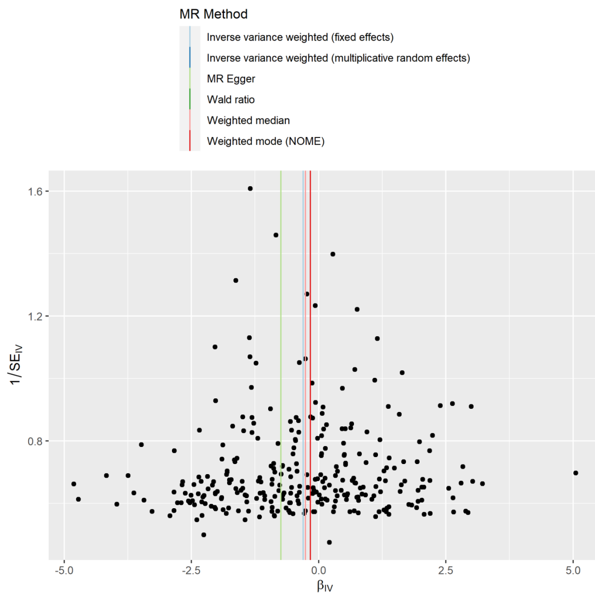
Fig.S14 Funnel plot of SNPs associated with education and their risk of ER- (Oncoarray)
