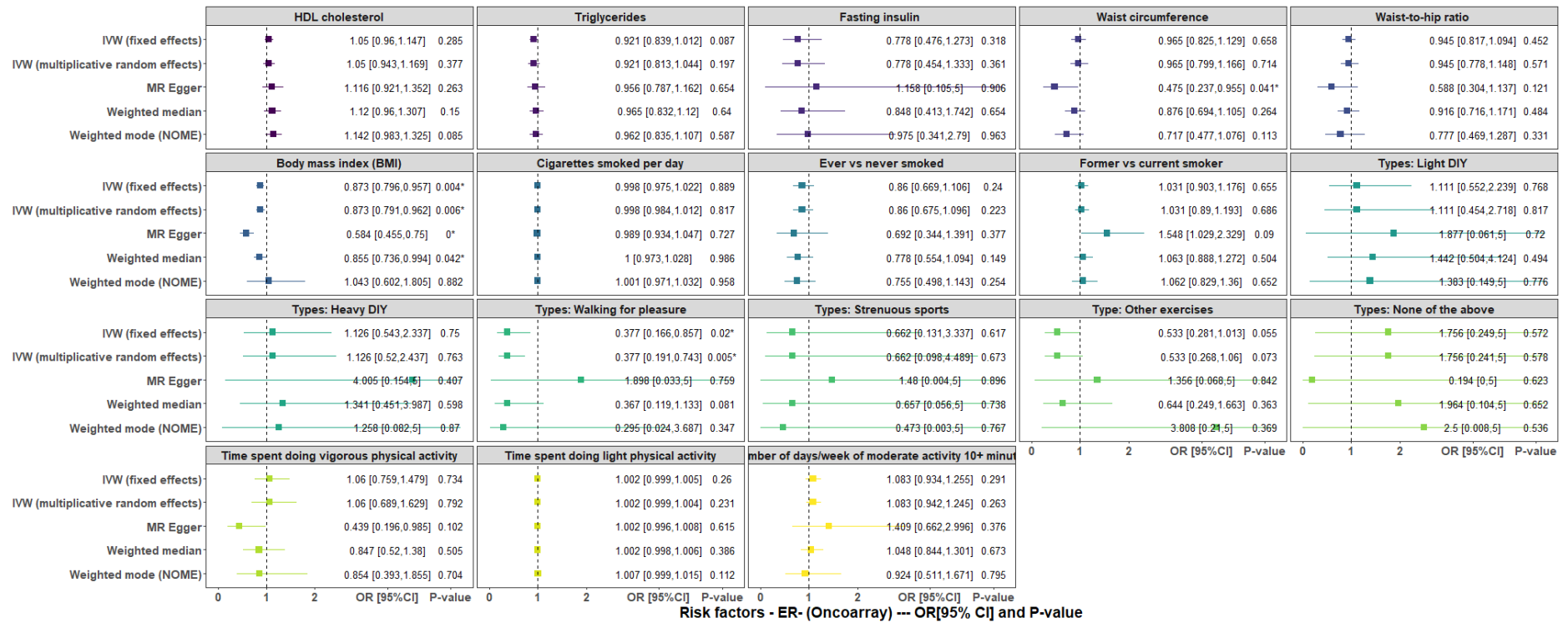
Fig.S6 Causal estimates of potential mediators on ER- (Oncoarray)
