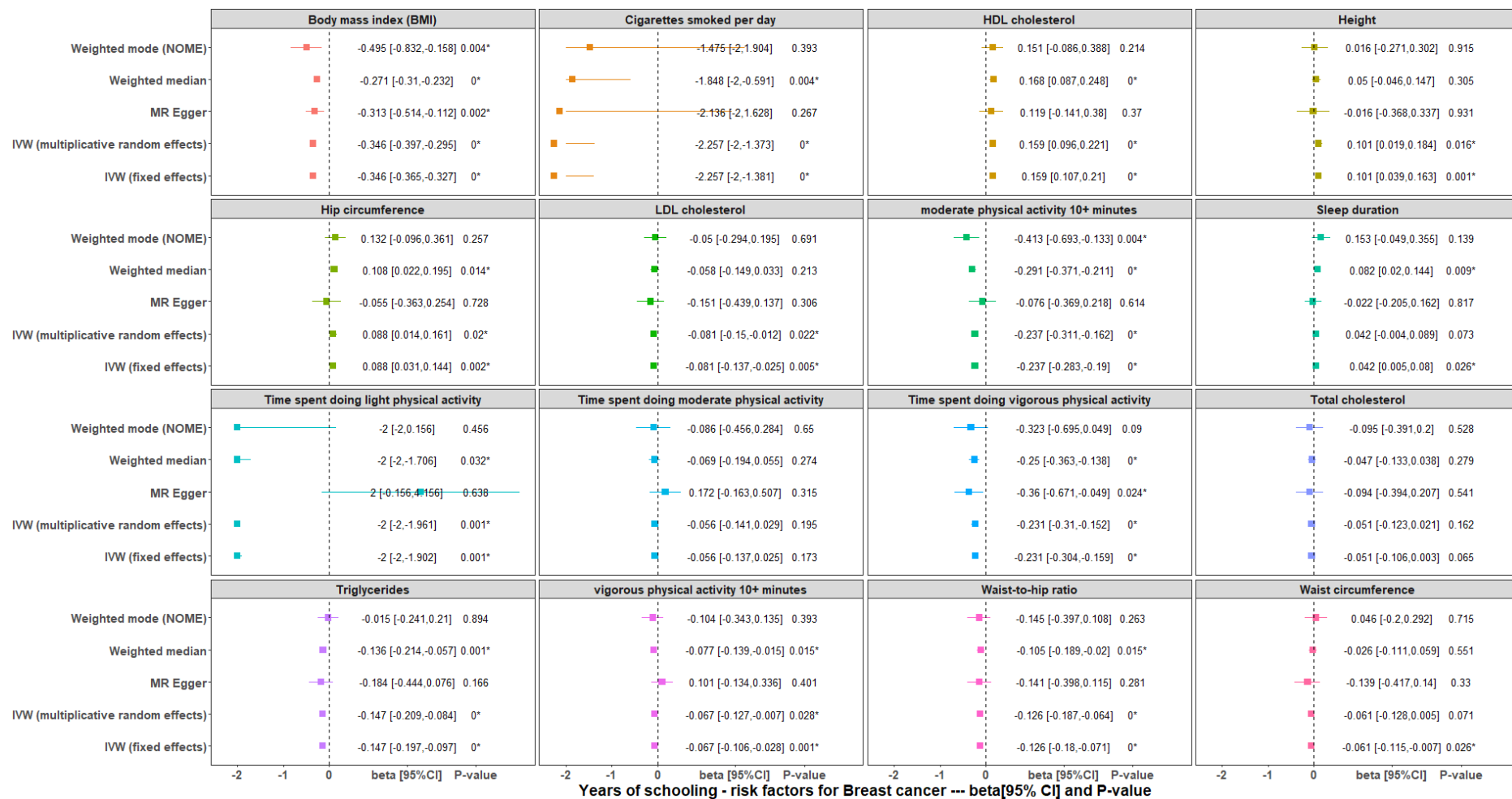
Fig.S2 Causal estimates of education on potential mediators (continue)
