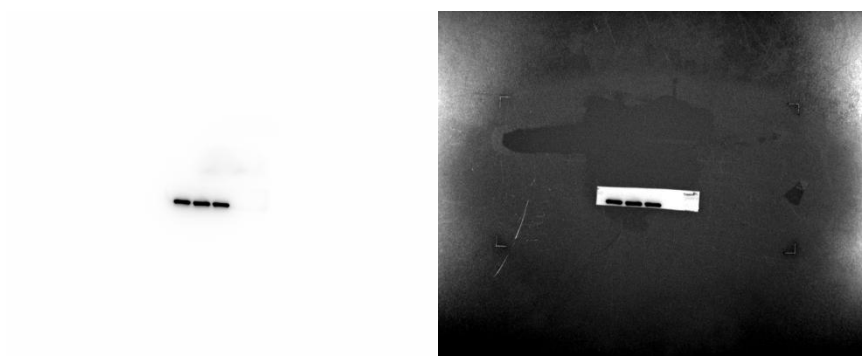
\beta -actin
