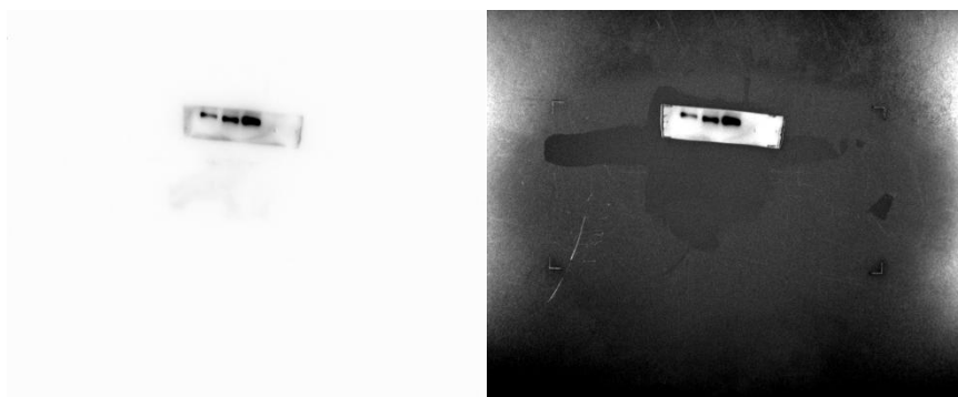
\beta -actin
