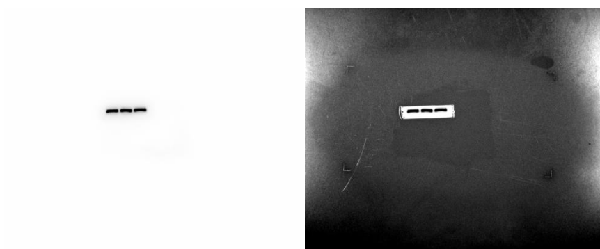
T24 β-actin
