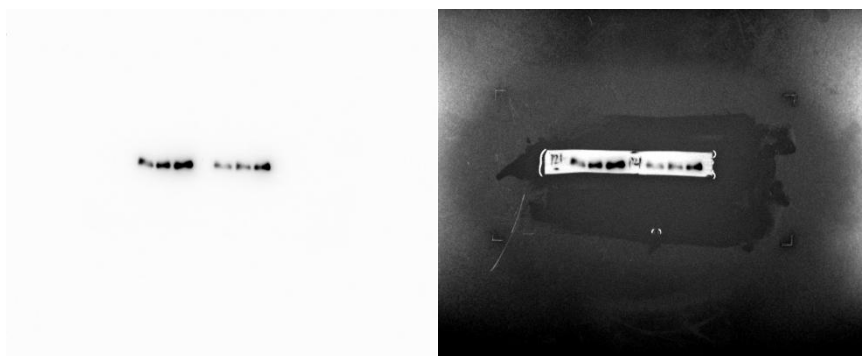
T24 β-actin
