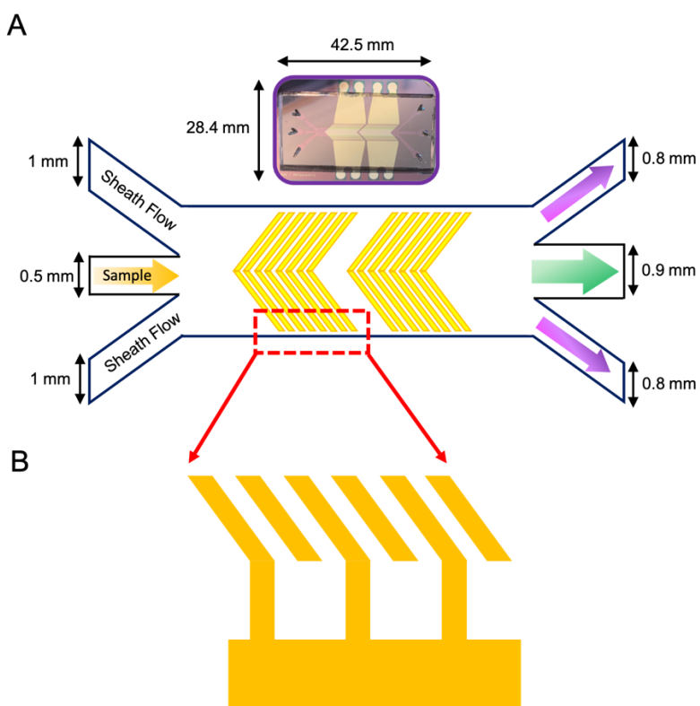
Figure S1. (A) Schematic of the microfluidic dielectrophoretic sorting device and real image of the device (top). (B) Electrode were designed interdigitatedly, half electrodes were connected to the bottom electrode pads, the other half were connected to the top electrode pads.
