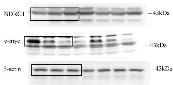
Figure 5C HeLa :
