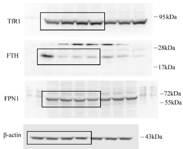
Figure 1 HeLa :
