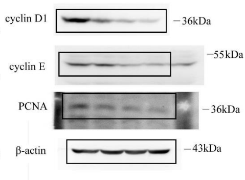
Figure 3B SiHa :
