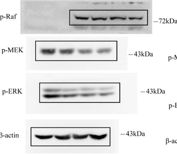
Figure 6 HeLa :
