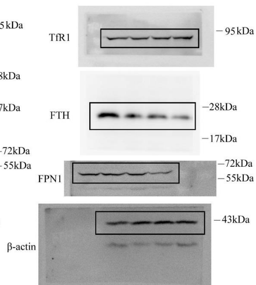
Figure 1 SiHa :
