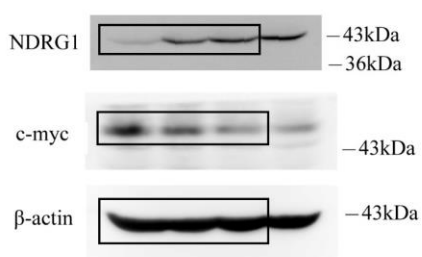
Figure 5C SiHa :
