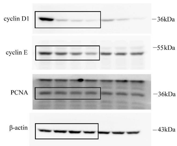
Figure 3B HeLa :
