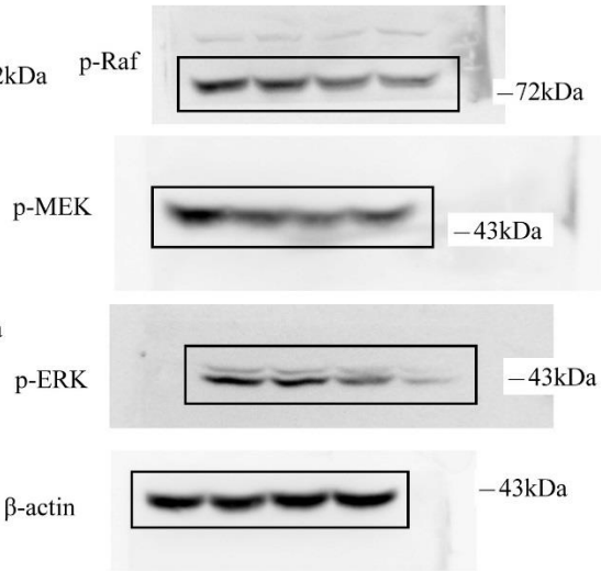
Figure 6 SiHa :
