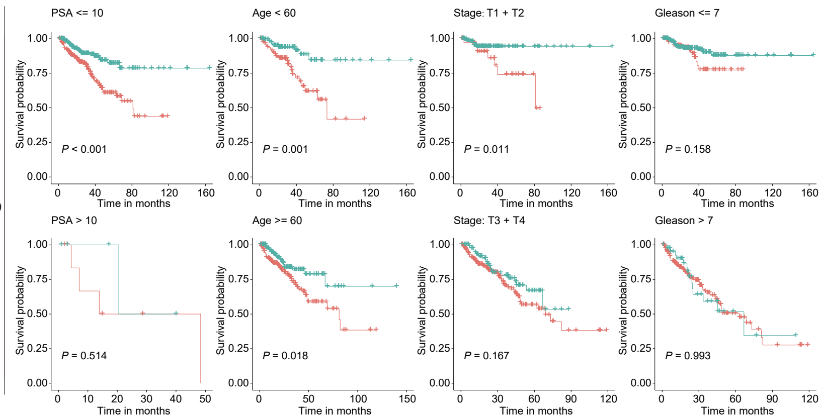
Figure S1. Kaplan-Meier analyses showed the usage of the eleven-consensus-gene-based classifier in different clinicopathological subgroups in GSE70768, TCGA-PRAD, and GSE116918 cohorts. Survival probability reflected the recurrence-free survival, P value obtained from the log-rank test.
