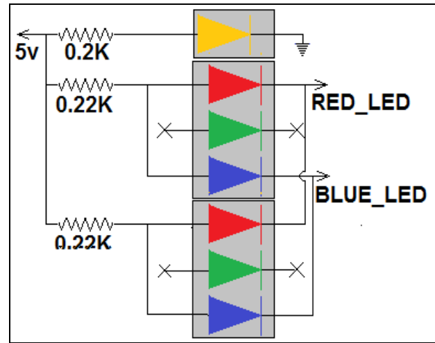
Schematic
