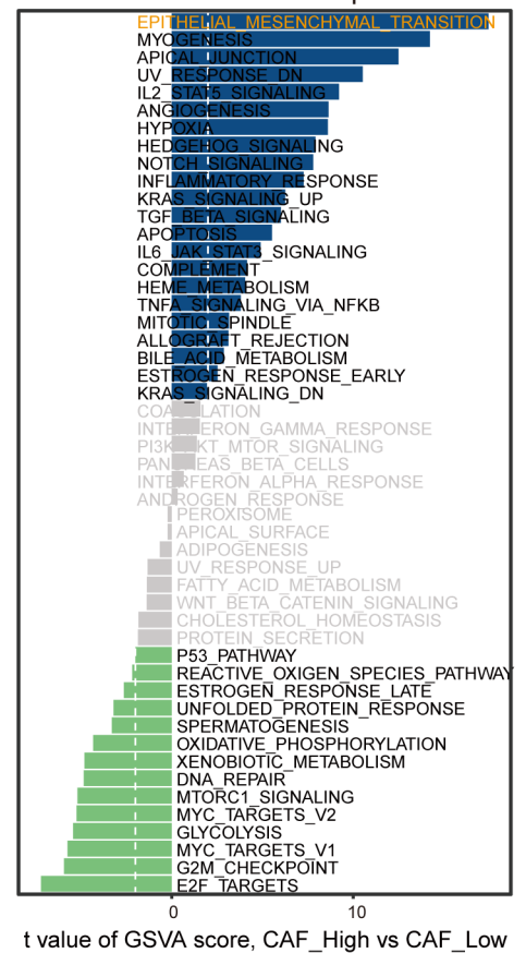
GSE15459 samples
