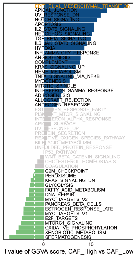
TCGA samples
