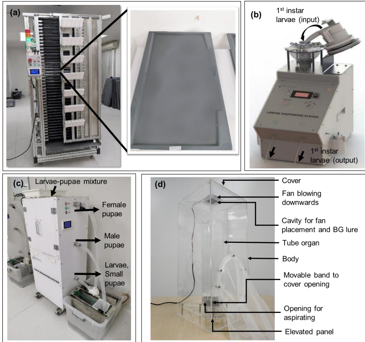
Supplementary Figure 2. Images of High Density Rearing Rack (HDRR) with High Density Rearing Tray (a), Larvae Dispensing System (b), Pupae Separation System (PSS) (c), Flight Test Device (FTD) (d).
