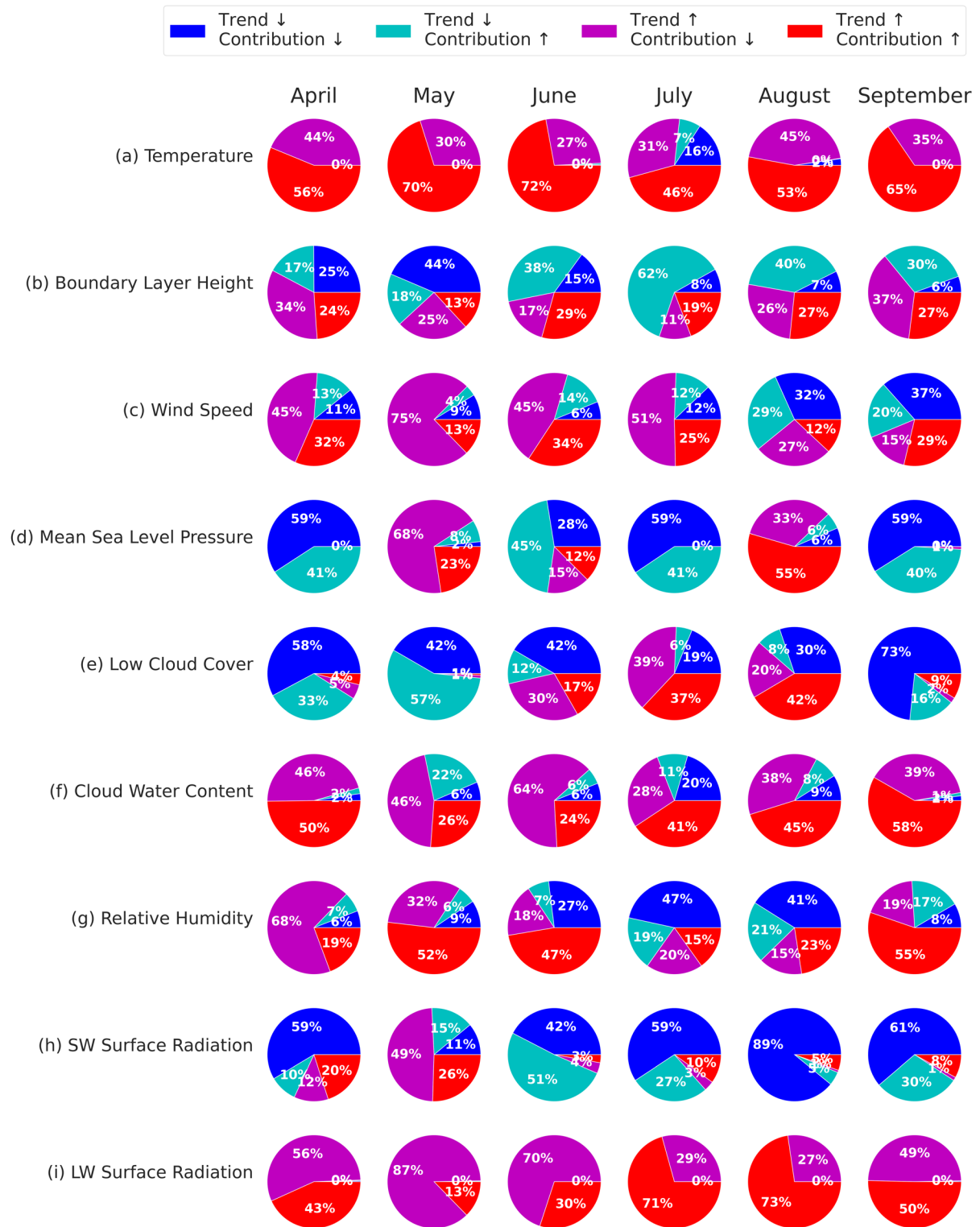
Figure S14. Results of the classification of each grid cell with an SS trend for each feature (rows) and each month (columns).
