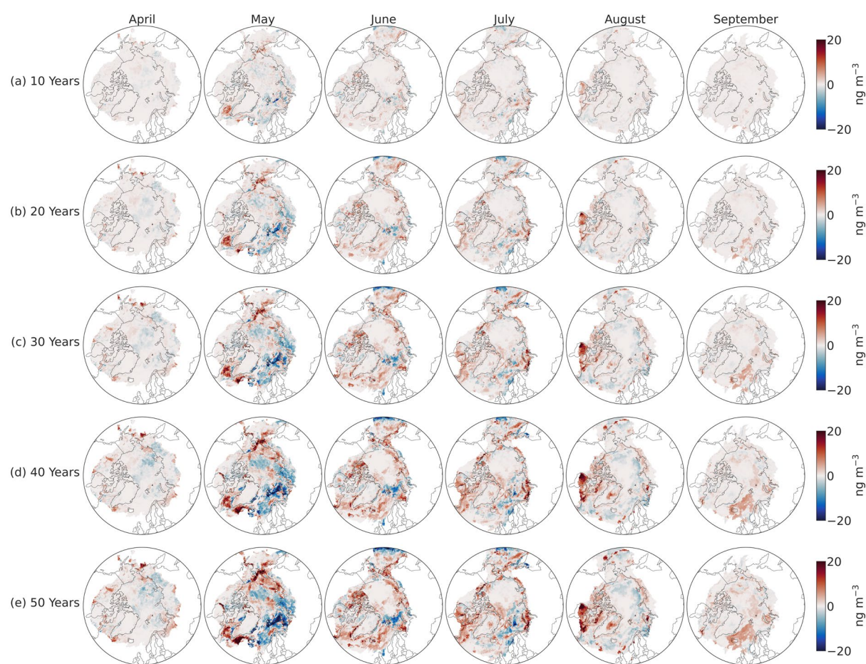
Figure S12. Maps of the projected absolute changes in MSA for each decadal interval compared to year 0 from our machine learning model.
