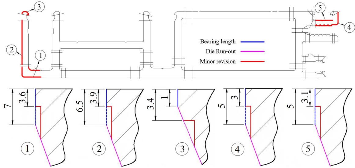
Figure 15. Detailed modifications in minor revision.
