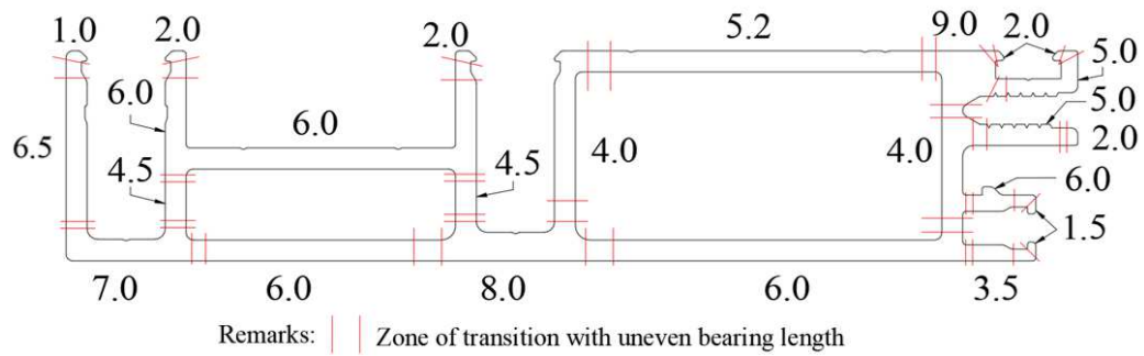
Figure 5. Bearing lengths of initial design (unit: mm).
