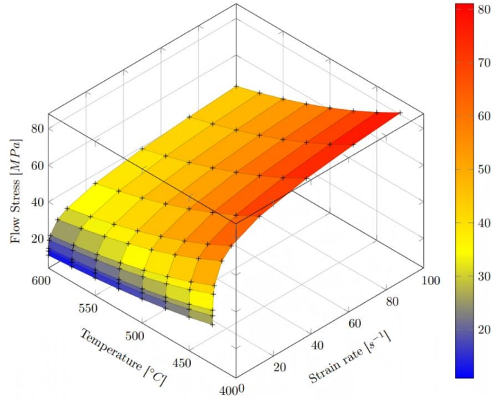
Figure 7. Flow stress [ \sigma = f(\dot{\epsilon}, T) ] data for AA7005.
