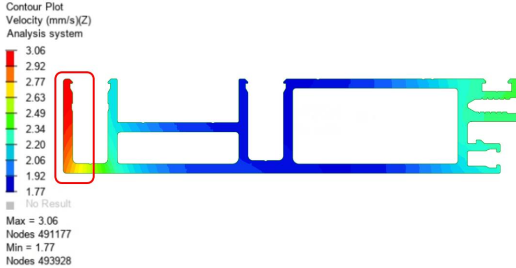
Figure 23. Velocity distribution at extrusion exit section of the major revision die.
