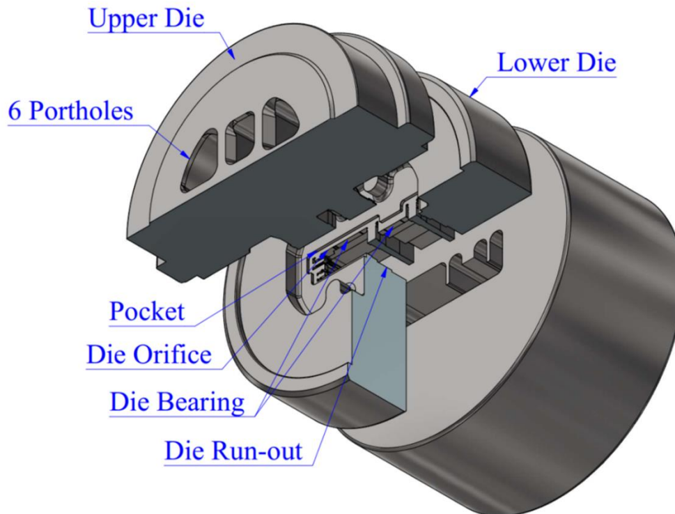
Figure 6. General outline of initial die design.
