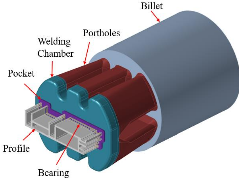
Figure 8. Simulation model for the porthole die extrusion process.
