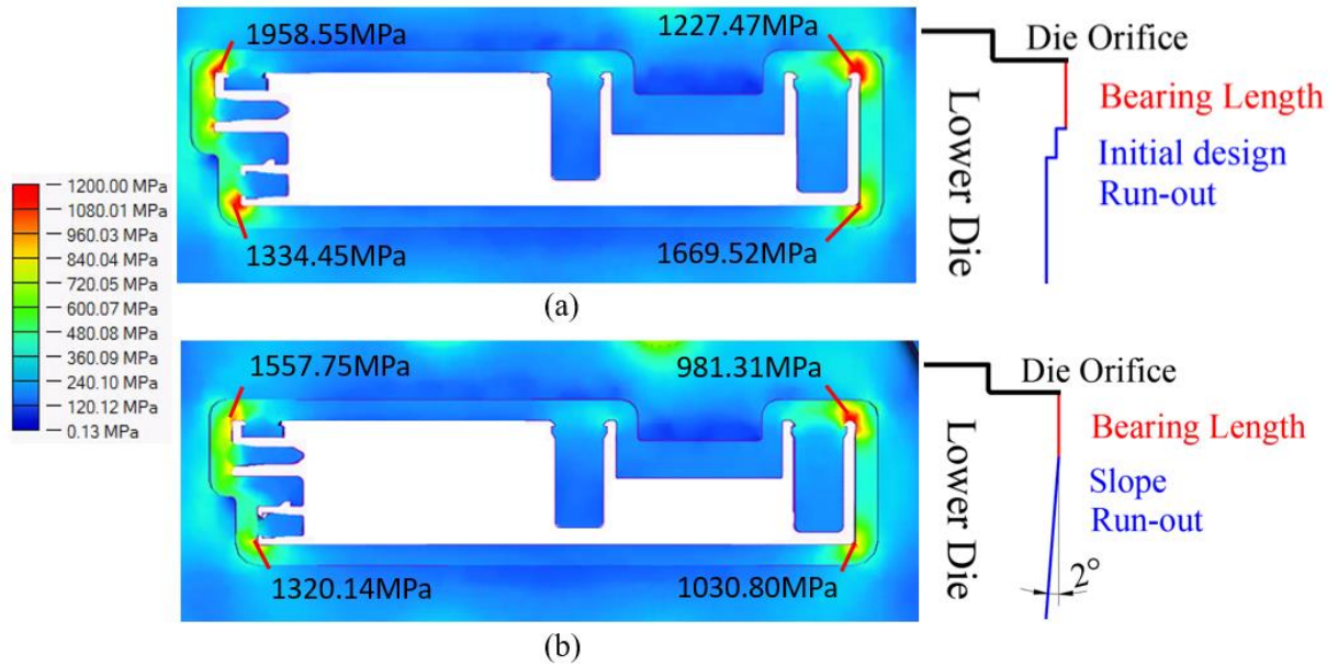
Figure 9. Steady-state die stress simulation results at ram speed of 0.1 mm/s. (a) Initial design run-out. (b) Slope run-out.
