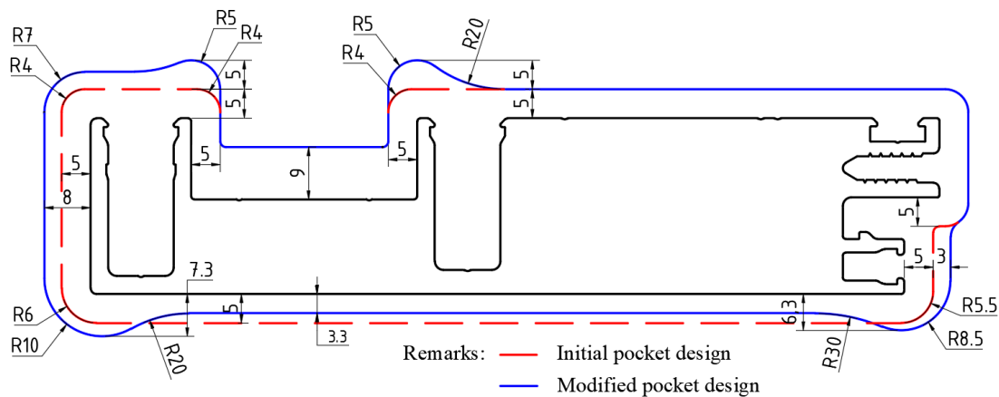
Figure 21. Comparison of original and modified pocket profiles.
