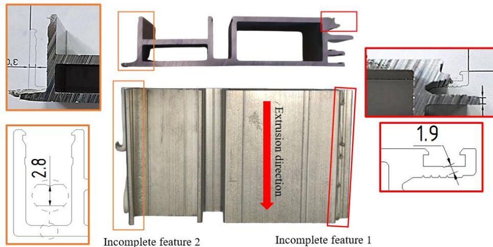
Figure 14. Cross-sections of extruded products and incomplete features in first extrusion trial.
