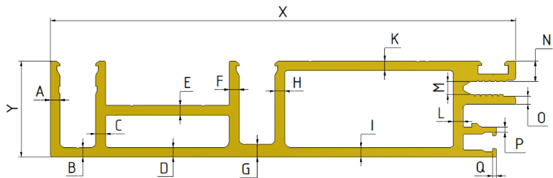
Figure 26. Dimensions of extrusion product.
