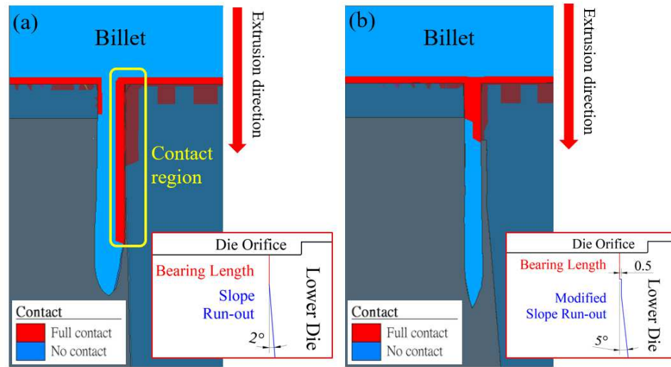
Figure 19. Runout contact simulation results of (a) initial design and (b) major revision.
