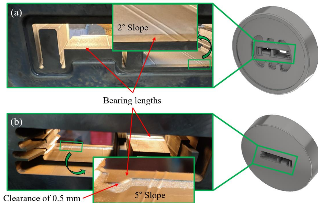
Figure 20. Design changes implemented in machined die (a) before and (b) after modification.
