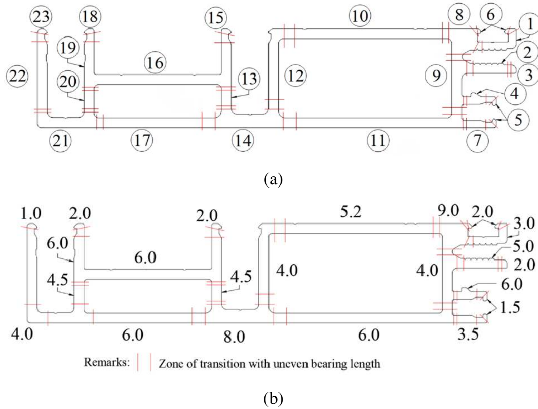
Figure 18. Bearing lengths. (a)Marked positions and (b) Major revision of bearing length.
