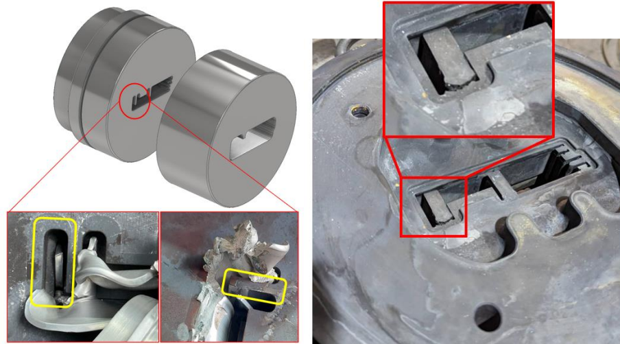
Figure 17. Severe blockage and irreparable damage of the lower die.
