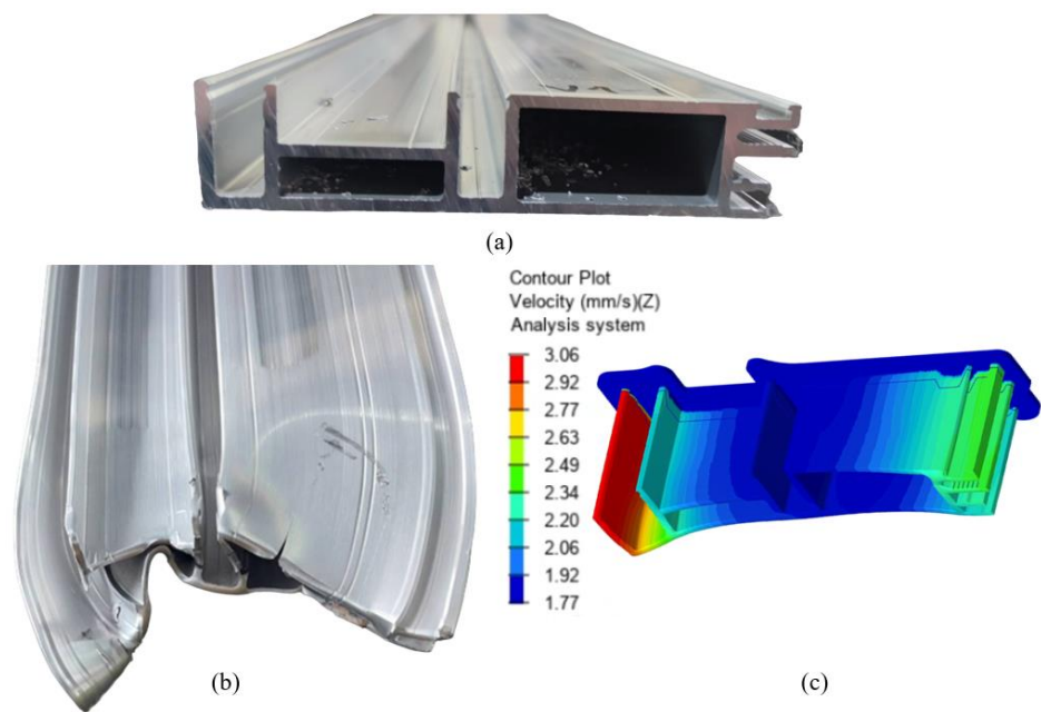
Figure 25. Experimental extrusion profile. (a) Final product. (b)Real front end. (c) Simulation front end.
