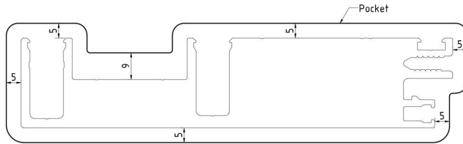
Figure 4. Pocket shape of initial design (unit: mm).
