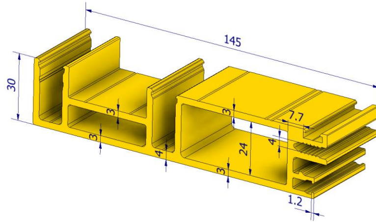
Figure 1. Dimensions of 3D model of desired profile (unit: mm).
