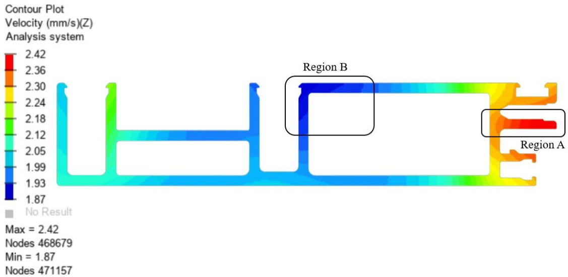
Figure 10. Velocity distribution on the cross-section of die exit for initial die design at ram speed of 0.1 mm/s.
