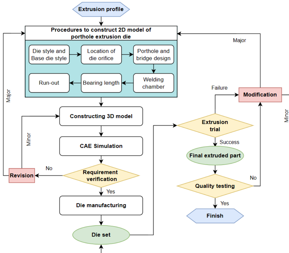
Figure 2. Flow chart of porthole die design process.
