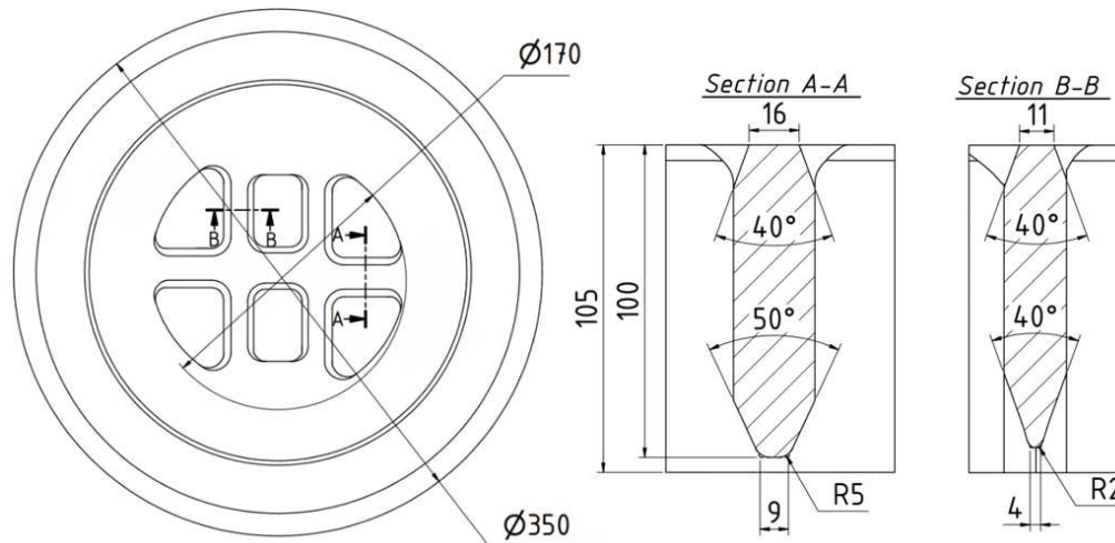
Figure 3. Structure of extrusion die bridge designed in present study.
