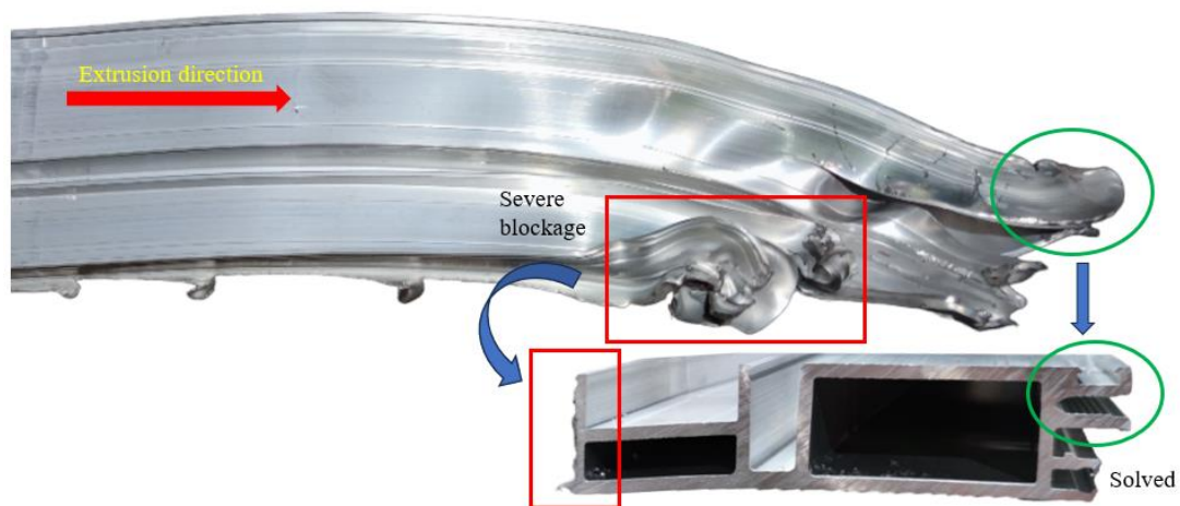
Figure 16. Front end and extruded profile obtained from the second extrusion trial.
