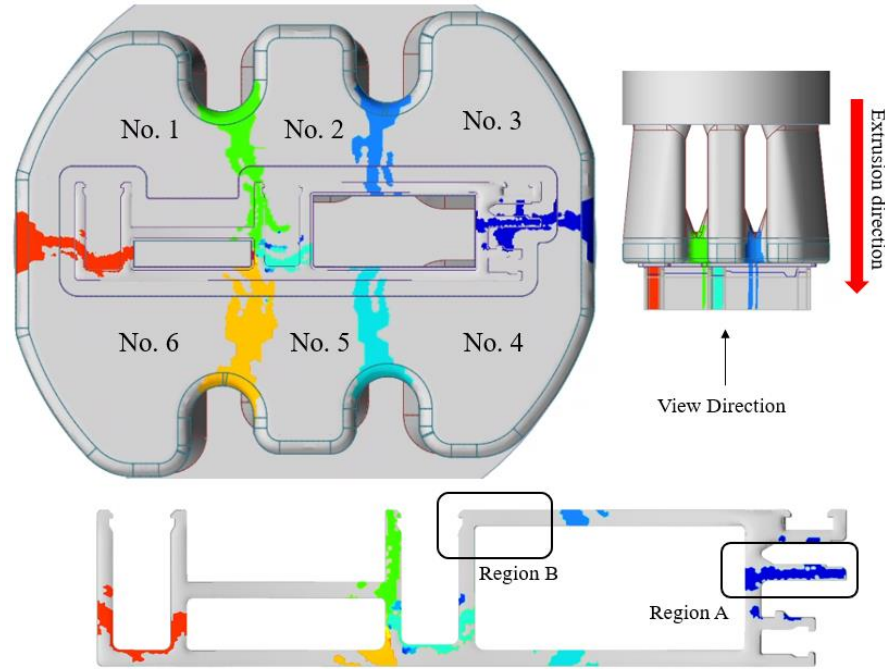
Figure 11. Location of portholes and simulation results of weld seams at ram speed 0.1 mm/s.
