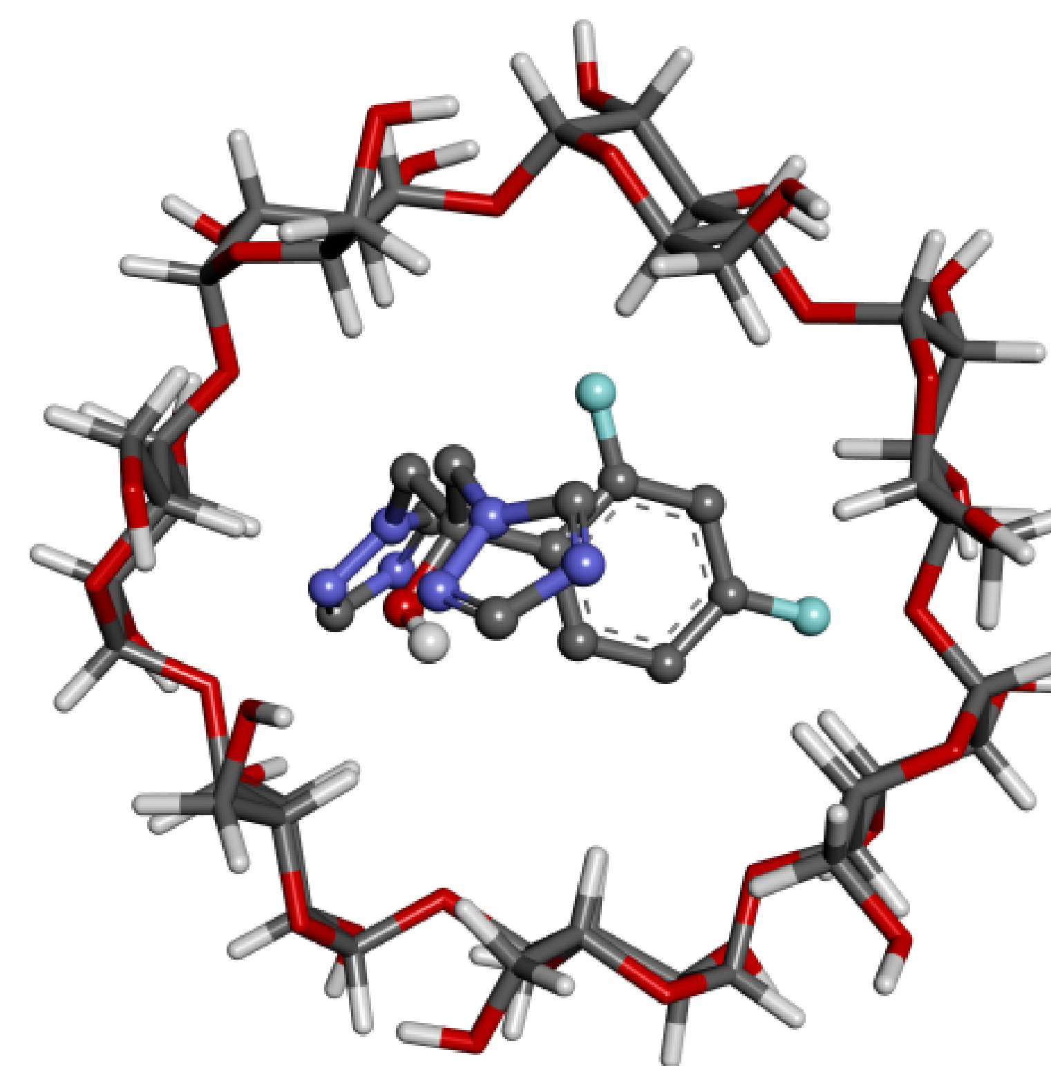
FCZ- \beta -CD1
