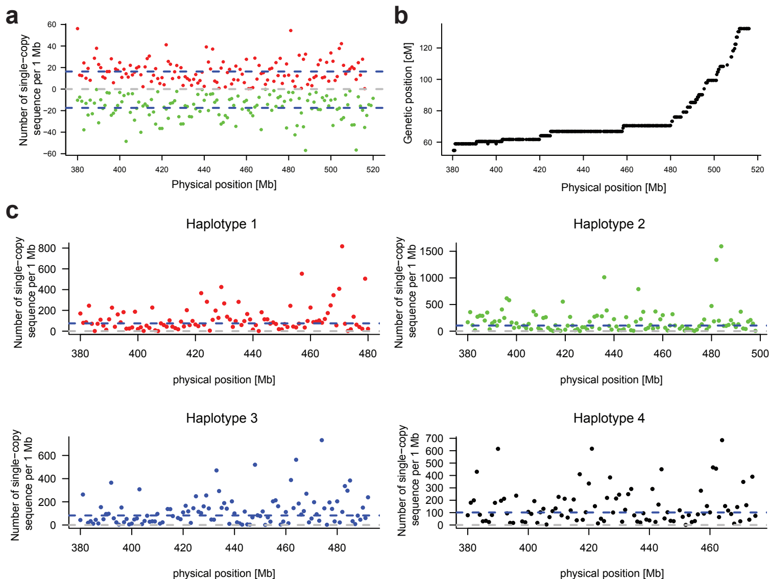
Extended Data Figure 3. Design of oligo-FISH probes. (a) Haplotype-specific single-copy sequence in 1 Mb bins at the distal end of the long arm of chromosome 5H in FB19-011-3. (b) Relationship between the genetic and physical maps of the long arm of chromosome 5H. (c) Haplotype-specific single-copy sequence in 1 Mb bins at the distal end of the long arm of chromosome 5H in FB19-028-3.
