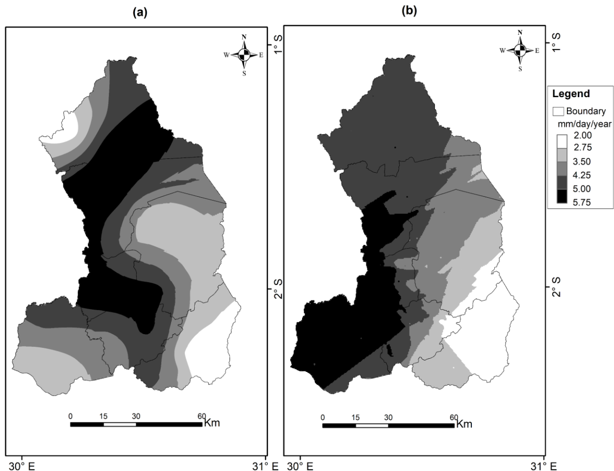
Fig. S1: Spatial distribution of MAM (a) and SON (b) mean rainfall for the period of 1981 to 2021.
