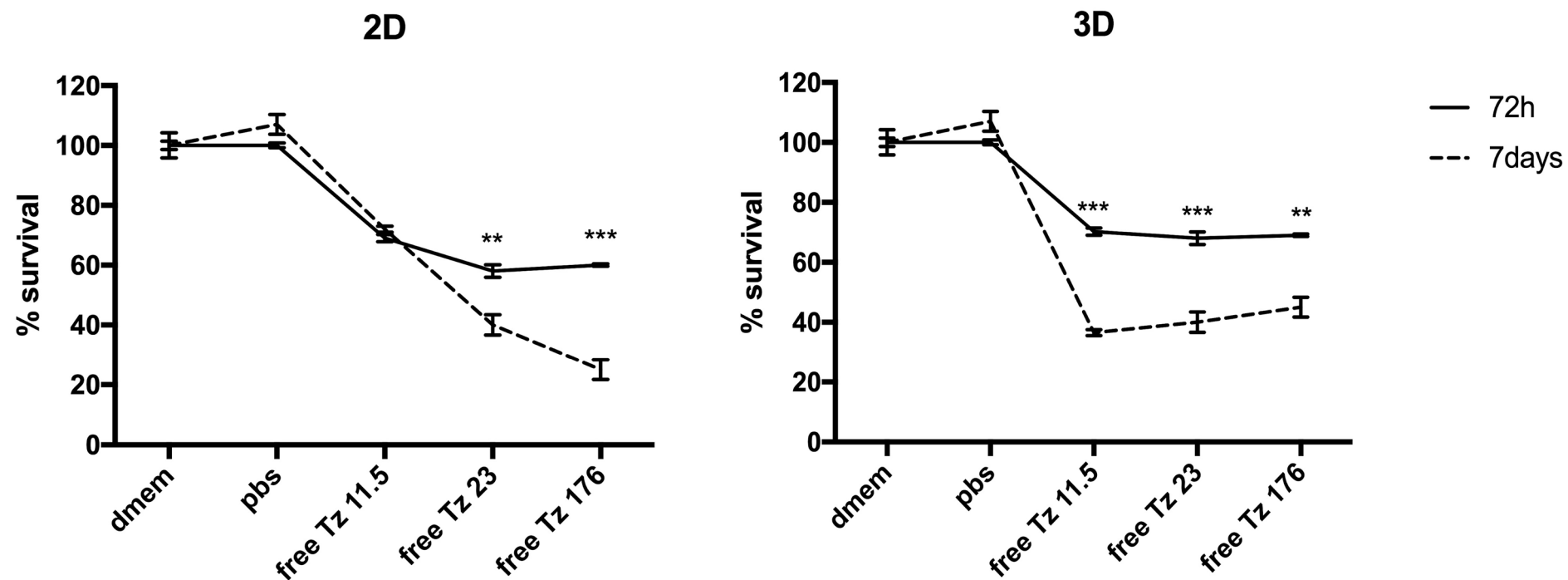
Figure S3. Efficacy of free TZ on cell proliferation inhibition in BT-474 cell line after 72 hours or 7 days of treatment in 2D and 3D culture models. ** p < 0.01 , *** p < 0.001 compared to untreated controls.
