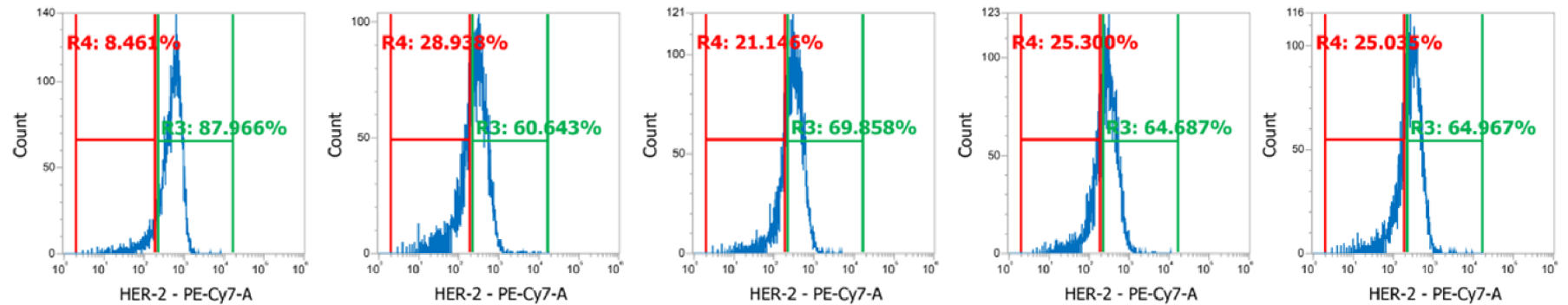
Figure S5. Flow cytometry analysis of HER2 expression in BT-474 cell line untreated (CTRL), treated with different PLGA+TZ nanoparticles or treated with free TZ after 72 hours or 7 days.
