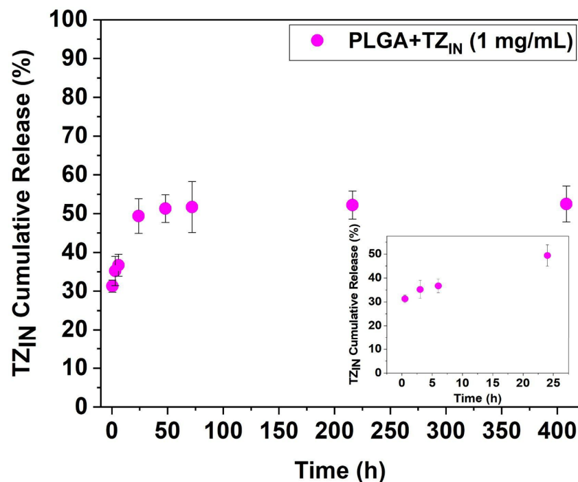
Figure S2. Cumulative release profile of trastuzumab. a) TZ released from PLGA nanoparticles, which encapsulate the mAB inside its aqueous core (PLGA+TZ IN ); b) TZ released from PLGA with empty core and subsequently functionalized on its surface with the TZ (PLGA+TZ OUT ). The experiments were performed three times in PBS buffer at 37°C for 14 days. The inset of figure a shows the percentage of drug release during the first 24 hours of incubation. The data are expressed as percentage of TZ released (amount of released over the total encapsulated TZ) vs time.
