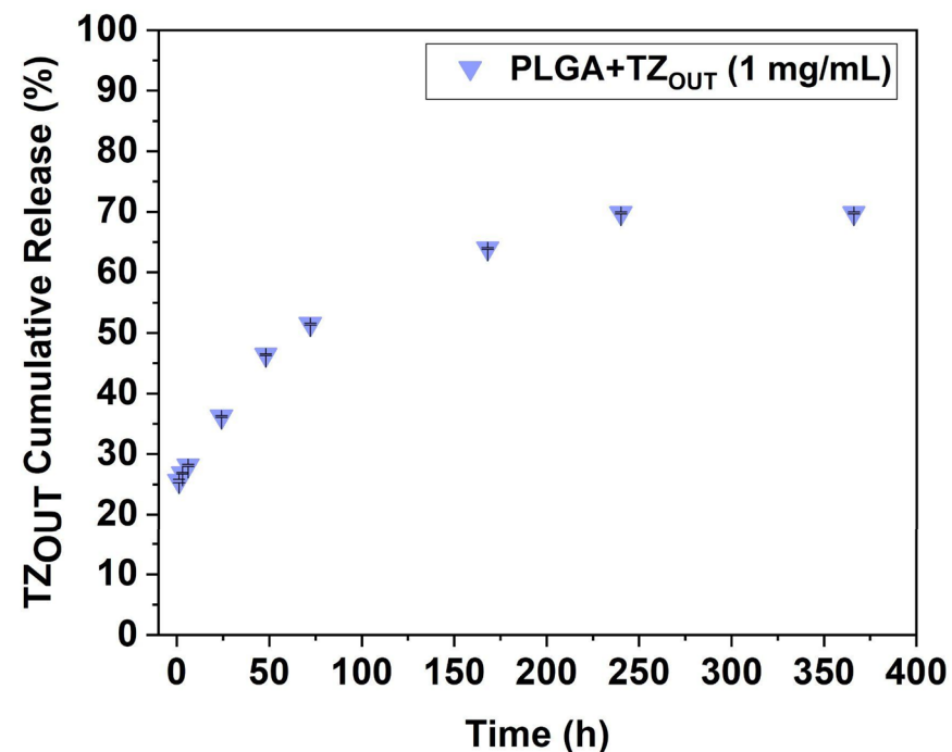
Figure S2. Cumulative release profile of trastuzumab. a) TZ released from PLGA nanoparticles, which encapsulate the mAB inside its aqueous core (PLGA+TZ IN ); b) TZ released from PLGA with empty core and subsequently functionalized on its surface with the TZ (PLGA+TZ OUT ). The experiments were performed three times in PBS buffer at 37°C for 14 days. The inset of figure a shows the percentage of drug release during the first 24 hours of incubation. The data are expressed as percentage of TZ released (amount of released over the total encapsulated TZ) vs time.
