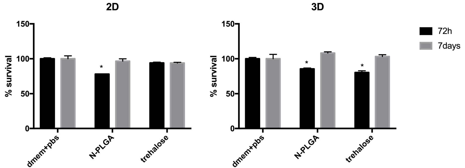
Figure S4. Effect of naked PLGA (N-PLGA) and trehalose on cell proliferation inhibition in BT-474 cell line after 72 hours or 7 days of treatment in 2D and 3D culture models. * p < 0.05 , compared to untreated controls.
