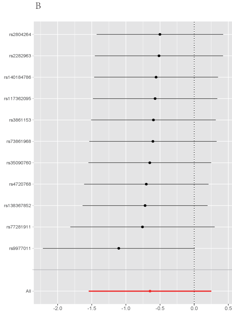
Supplementary Figure S31. Forest plot (A), Leave-one-out plot (B), scatter plot (C) and funnel plot (D) of the causal effect of mania on NAFLD.
