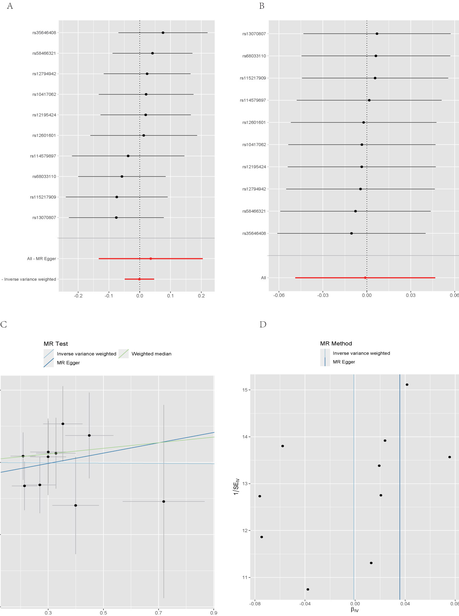
Supplementary Figure S4. Forest plot (A), Leave-one-out plot (B), scatter plot (C) and funnel plot (D) of the causal effect of Obsessive-compulsive disorder on NAFLD.
