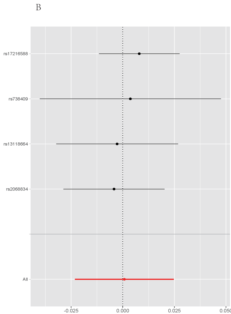
Supplementary Figure S41. Forest plot (A), Leave-one-out plot (B), scatter plot (C) and funnel plot (D) of the causal effect of NAFLD on Major Depressive Disorder.
