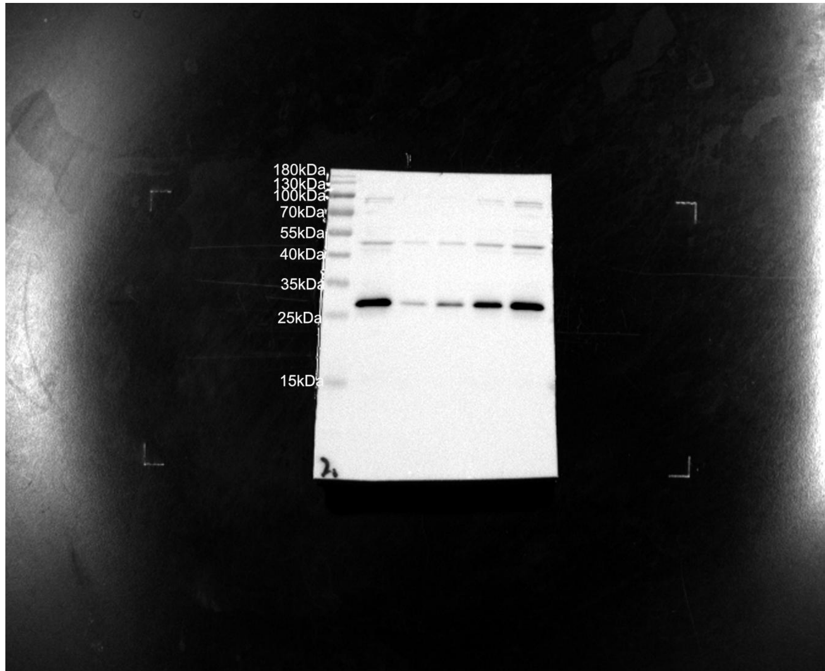
Fig1C-Bcl-2
