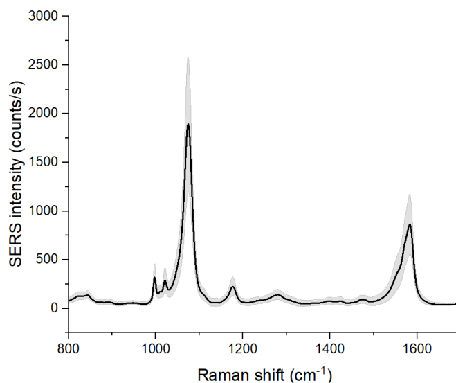
Figure S2 Average spectra of 4-MBA SERS signals.
