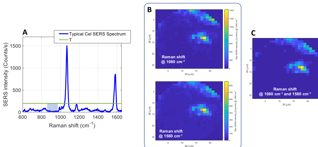
Figure S3 Workflow for determining the “number of pixels” in a SERS map. A) SERS positive control spectra highlighting the threshold set, B) Raw data SERS intensity maps corresponding to 1080 (upper panel) and 1580 \text{cm}^{-1} (lower panel) peaks, C) Intensity map considering the number of pixels with intensity above the threshold.
