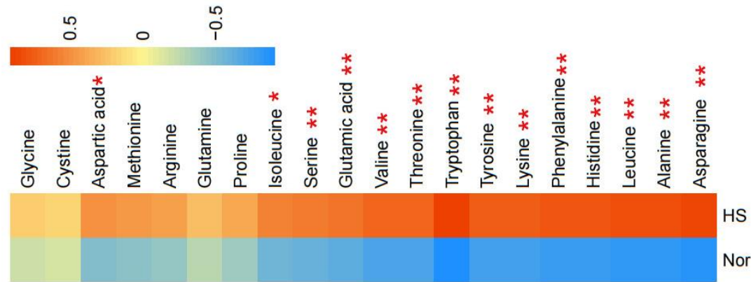
FigS2. Twenty amino acids in colonic contents. A: Twenty amino acids, B: Area under curve of Twenty amino acids. Statistical analysis was performed using Student-t test, * p < 0.05, ** p < 0.01.
