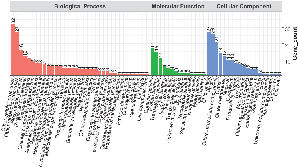
Cluster 3
