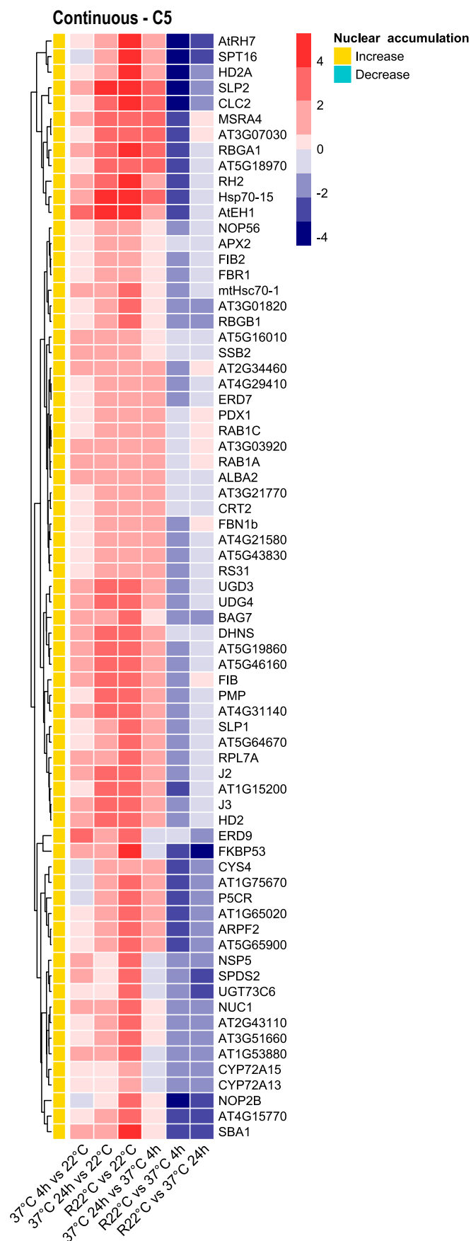
Figure S4D. Heat map. Heat maps show the \log_2 FC for every protein from Cluster C5 from Continuous Group (CIG) in indicated temperature/time comparisons. p values for 37°C 4 h vs 22°C=0.0005); 37°C 24 h vs 22°C=0.001; R22°C vs 22°C=0.001), 37°C 24 h vs 37°C 4 h=0.0004, R22°C vs 37°C 4 h = 0.0007 and R22°C vs 37°C 24 h= 0.0005. FDR = 0.98-1.14%. Proteins whose nuclear abundance increases or decreases during exposure to 37°C are shown in yellow and blue respectively.
