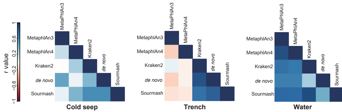
Fig. S1. Similarity between the profiles generated by the three reference-dependent profilers, the de novo assembling approach, and the k-mer profile produced by sourmash, with the intensity of the blue color denoting the strength of the correlation.
