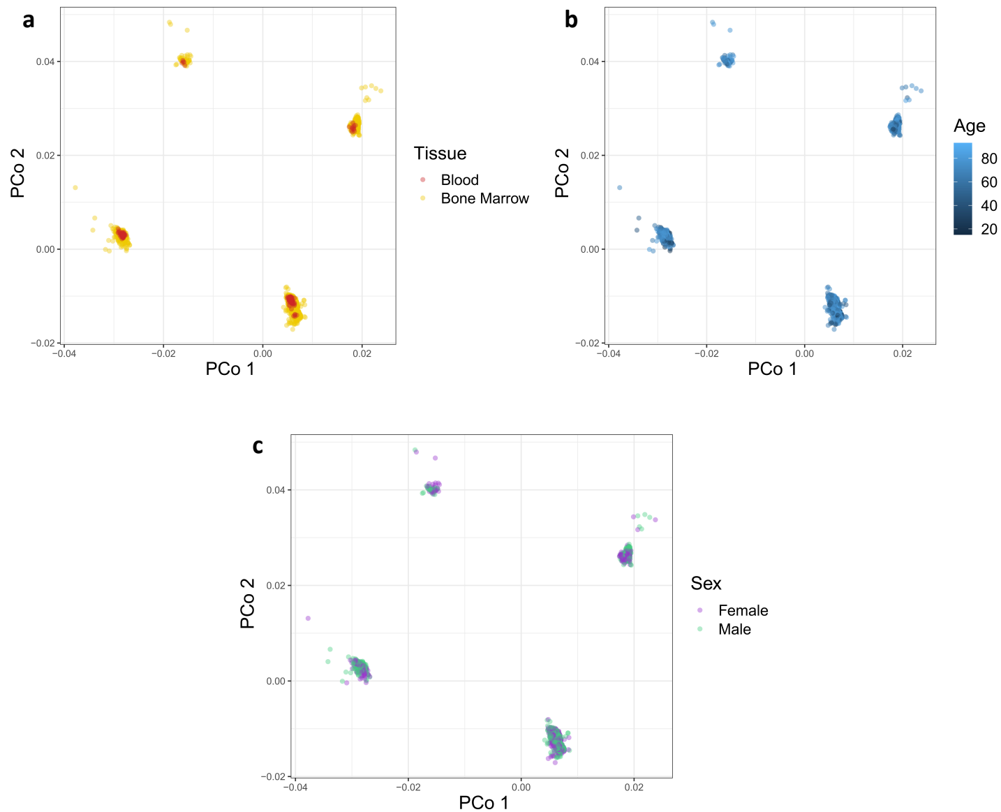
Supplementary Figure 2: Principal coordinate plots colored by sample characteristics. 1870 cases colored by a) blood/bone marrow status, b) age, and c) sex. For clarity, two outliers are not shown (bone marrow from males, ages 48 and 81).
