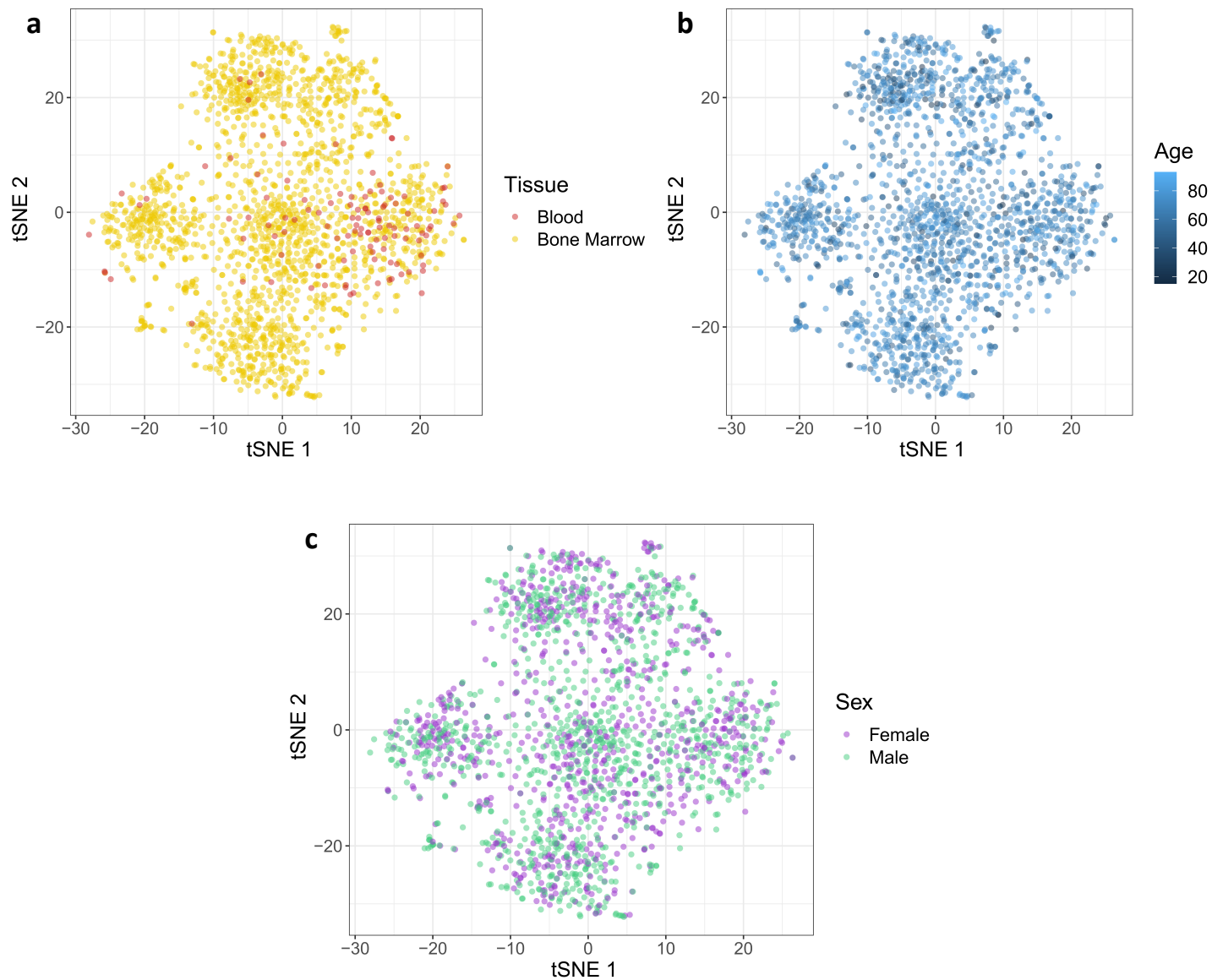
Supplementary Figure 1: t-SNE plots colored by sample characteristics. 1870 cases and 12 controls colored by a) blood/bone marrow status, b) age, and c) sex.
