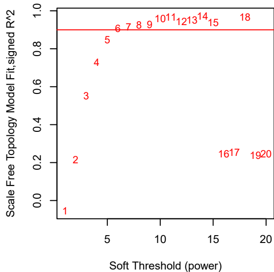
Scale independence
