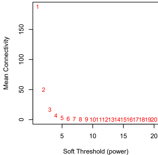
Mean connectivity
