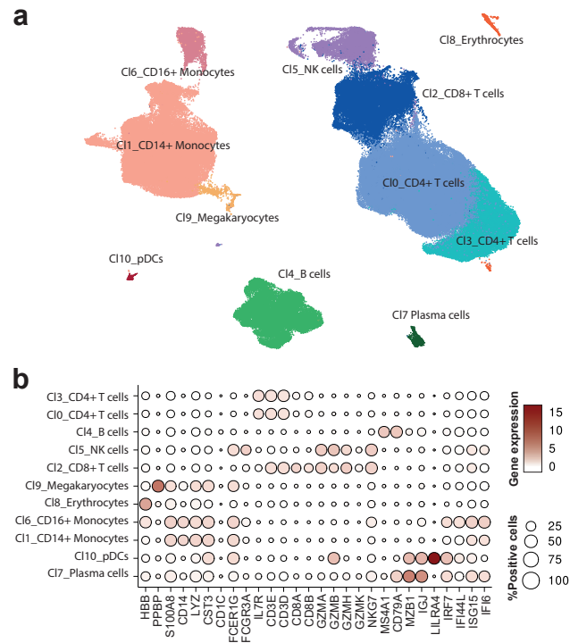
Supplementary Figure 5. Single cell clustering and major blood cell type identification. a , UMAP representation of single cell clustering. Each dot represents a cell, and cells belonging to the same cluster are colored with the same color. b , Gene expression of the major blood cell type markers across the different clusters. Color scale represents expression magnitude and circle size represents the percentage of cells within a cluster that express a certain marker.
