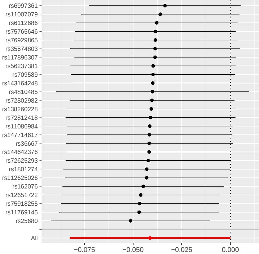
MR leave-one-out sensitivity analysis for 'CD27 on unswitched memory B cell' on 'Endometrial cancer || id:ebi-a-GCST00646
