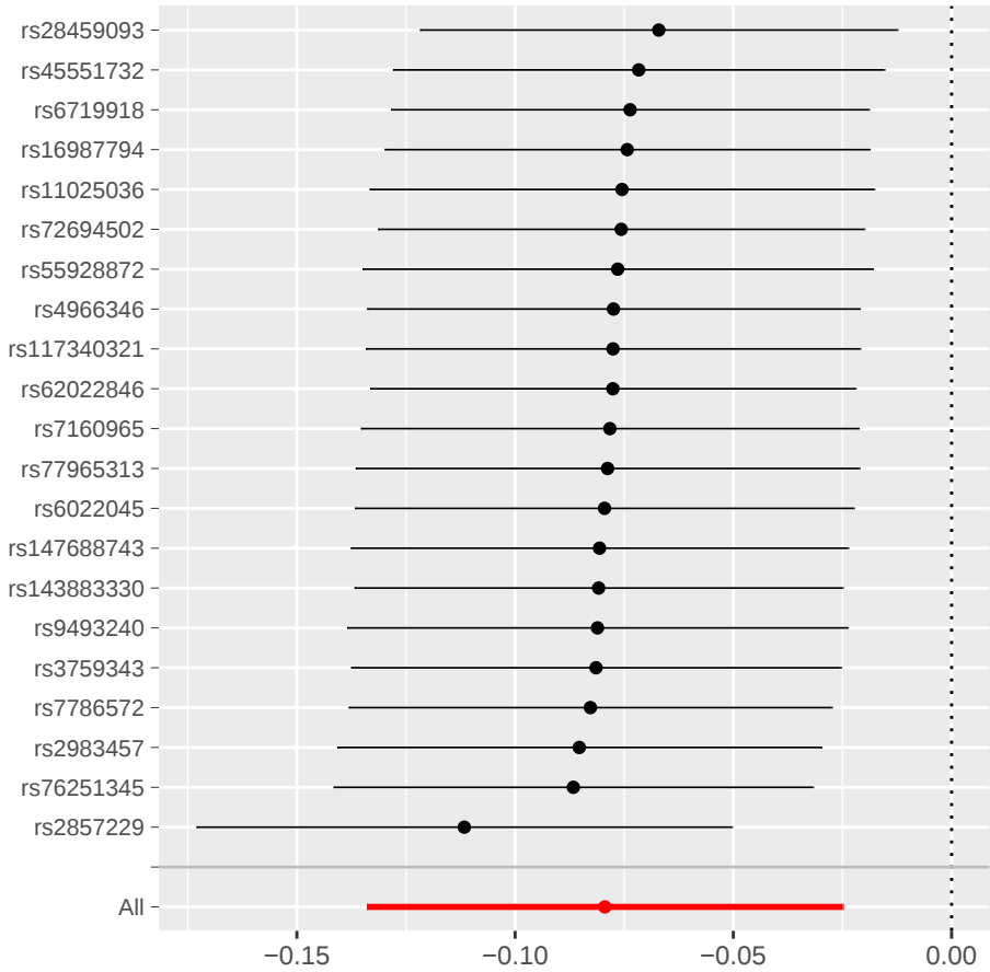
MR leave-one-out sensitivity analysis for 'CD4+CD8+ T cell %leukocyte' on 'Endometrial cancer || id:ebi-a-GCST006464'
