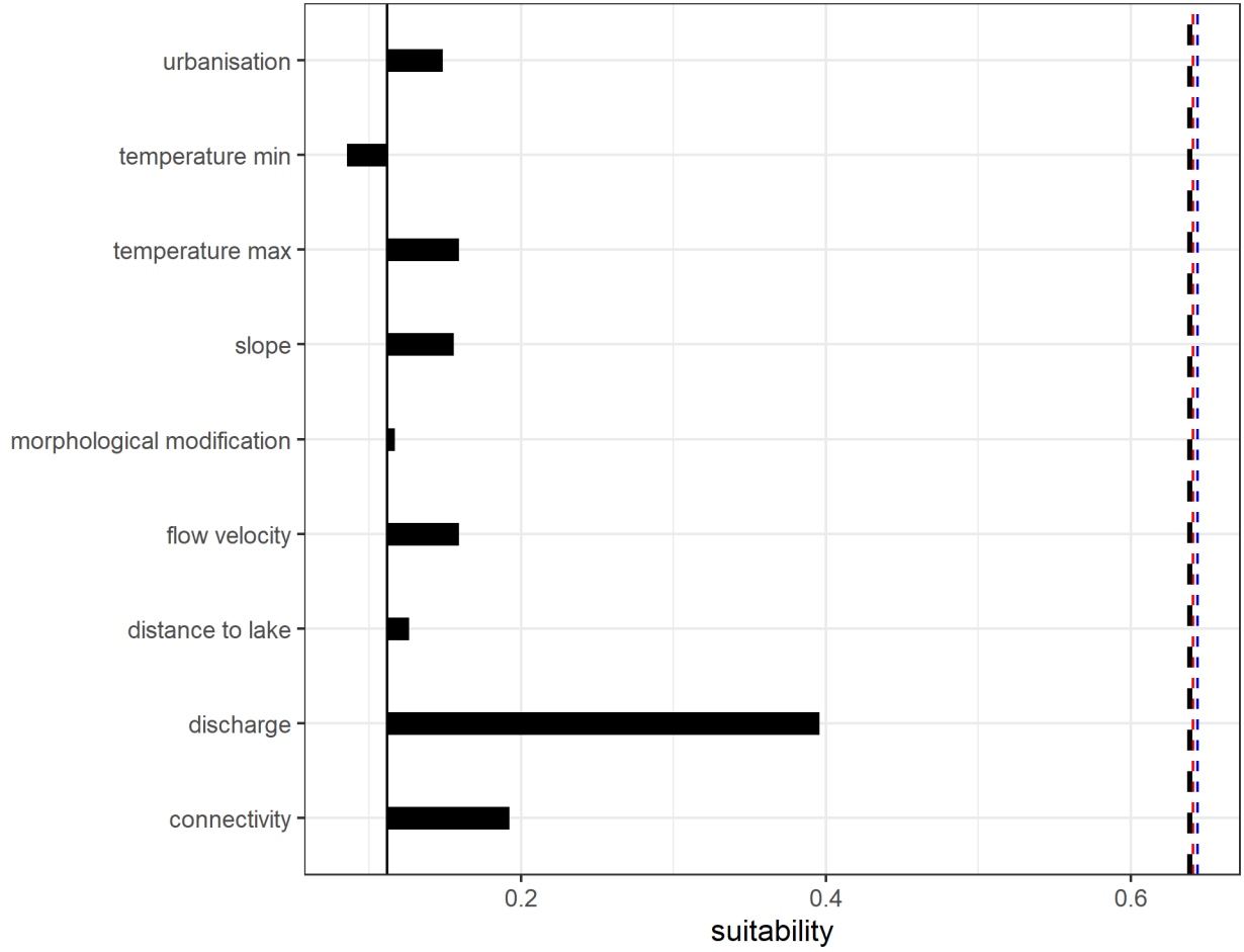
Figure 11. Shapley contributions to model local prediction (dashed lines) expressed as deviation from baseline model prediction. Red and blue dashed lines indicate the summed Shapley values + baseline prediction for fastshap (blue) and SHAP (red) methods, giving almost identical results.
