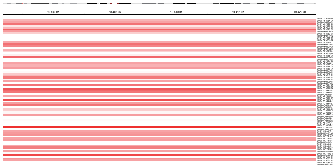
Figure S1. TFAP2A was amplified in UM
