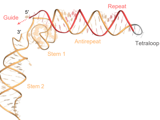
NmCas9 (PDB: 6JDV)
