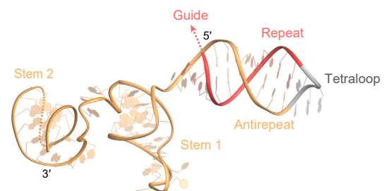
St1Cas9 (PDB: 6RJD)
