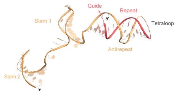
St1Cas9 (PDB: 6RJD)
