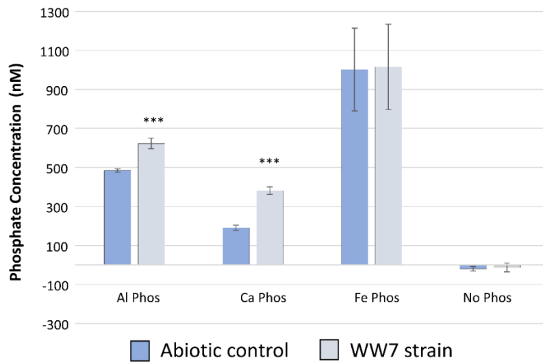
Figure S1. Aluminum Phosphate (Al Phos), Calcium Phosphate (Ca Phos), Iron Phosphate (Fe Phos) solubilization assay in strain WW7. No Phosphate (No Phos) condition was used as negative control. Bars and error bars represent the average and standard deviation of 4 independent measurements. Significance values of the T-test are * p < 0.1 ; ** p < 0.05 ; *** p < 0.01 .
