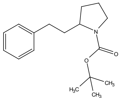
(±)-16 1 H NMR, 500 MHz, CDCl 3
