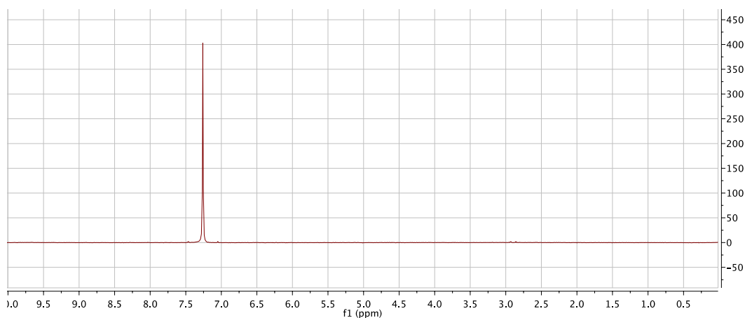
^2\text{H} NMR of reaction crude
