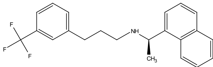
Sensipar ^{13}\text{C} NMR, 125 MHz, \text{CDCl}_3
