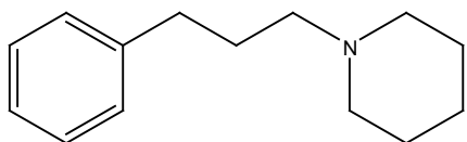
41 ^{13}\text{C} NMR, 125 MHz, \text{CDCl}_3
