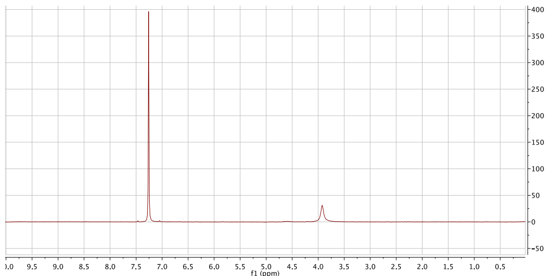
2 H NMR of product
