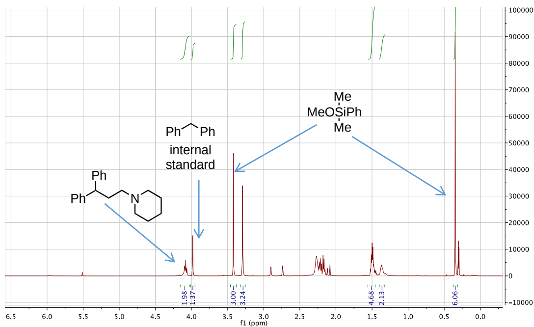
^1\text{H} NMR of reaction crude
