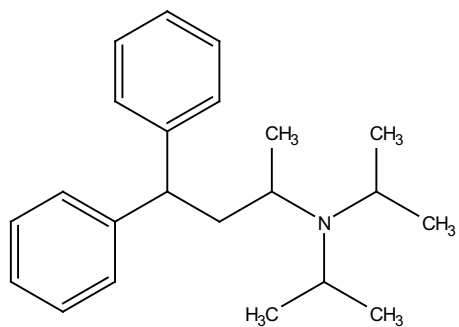
(±)-19 1 H NMR, 500 MHz, CDCl 3
