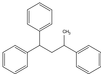
(±)-2 ^1\text{H} NMR, 400 MHz, \text{CDCl}_3
