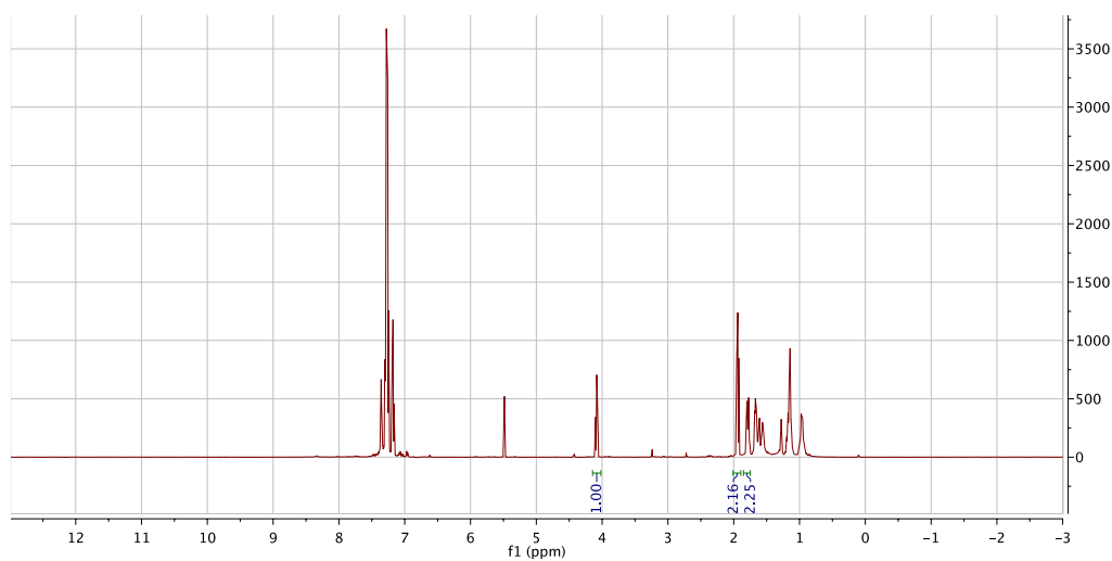
^1\text{H} NMR of reaction crude
