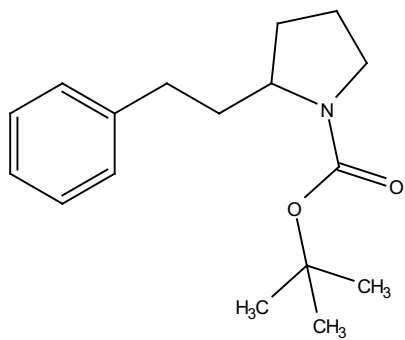
(±)-16 ^{13}\text{C} NMR, 126 MHz, \text{CDCl}_3
