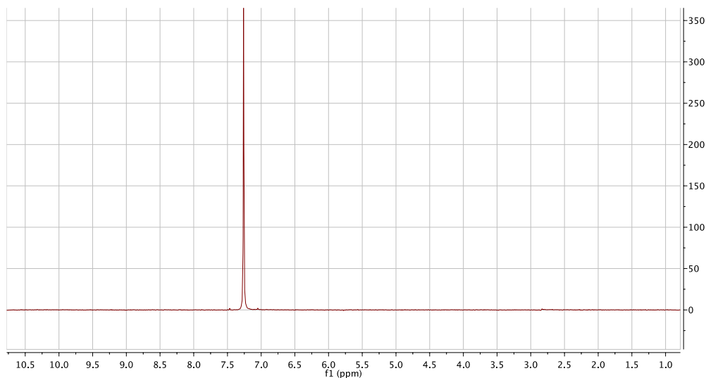
^2\text{H} NMR of reaction crude
