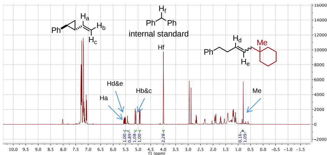
^1\text{H} NMR of reaction crude
