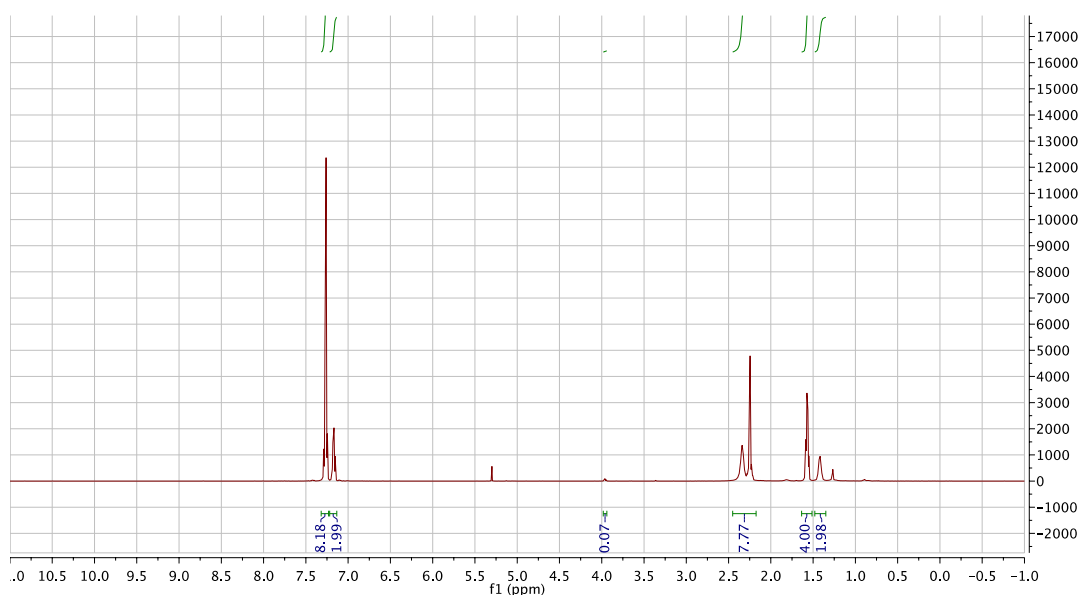
1 H NMR of product
