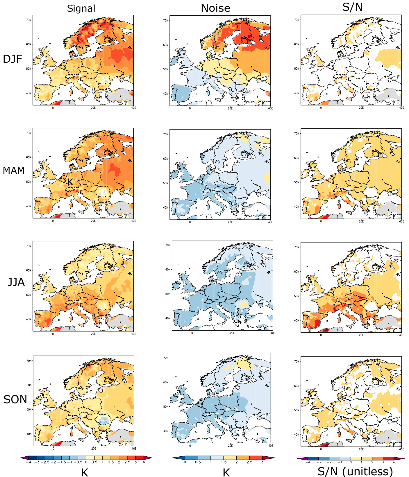
Figure S1: Signal (K), noise (K), and signal-to-noise ratio (S/N) of seasonally averaged surface temperature anomalies (1951-2016) in the EOBS V21 dataset. Grey regions indicate a lack of sufficient data. Stippling in the signal plots (left column) indicates signal values statistically significantly different from zero. Only S/N values statistically significantly from zero are shown (right column).
