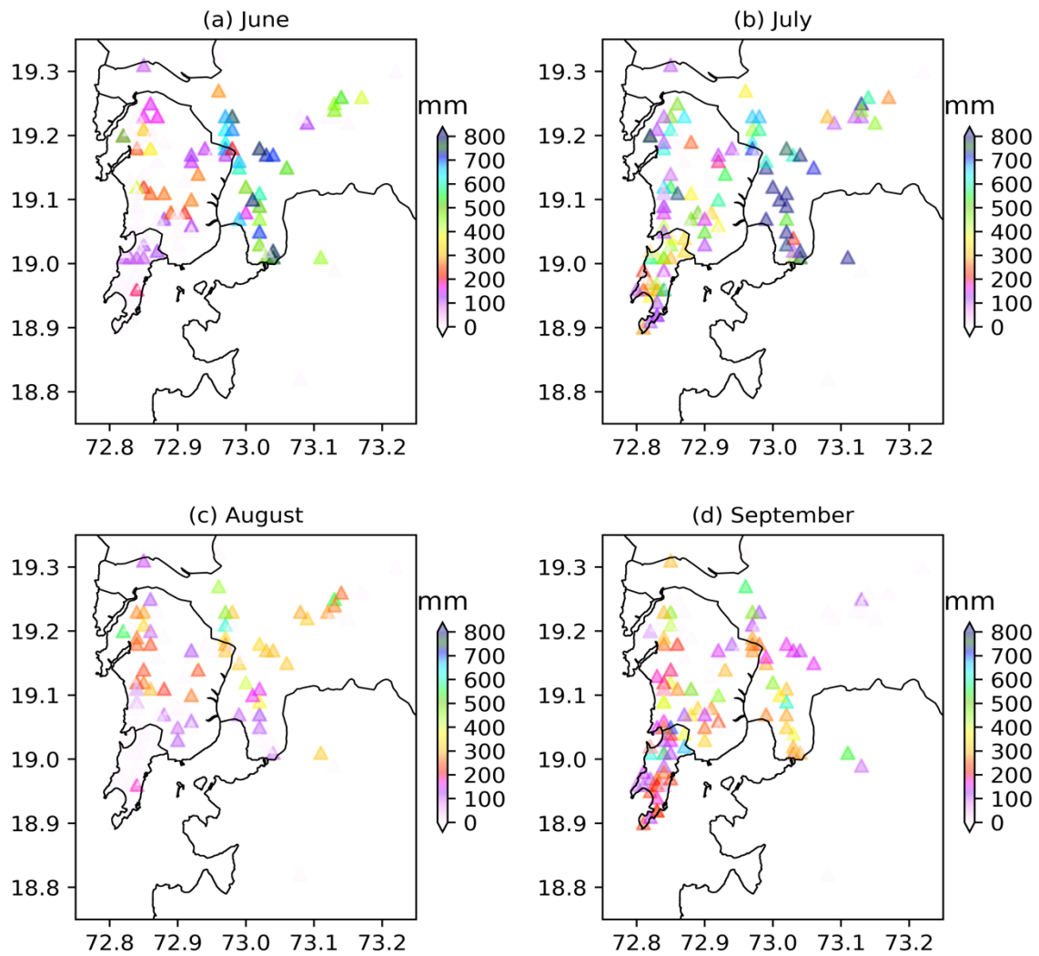
Figure S1: Monthly totals of rainfall from the ARG stations during 2019-2021 during (a) June, (b) July, (c) August and (d) September
