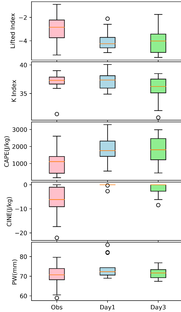
Figure S3: Box charts of thermodynamic indices (LI, K-index, CAPE, CINE and Pw) computed from observations and NCUM-reg forecasts.
