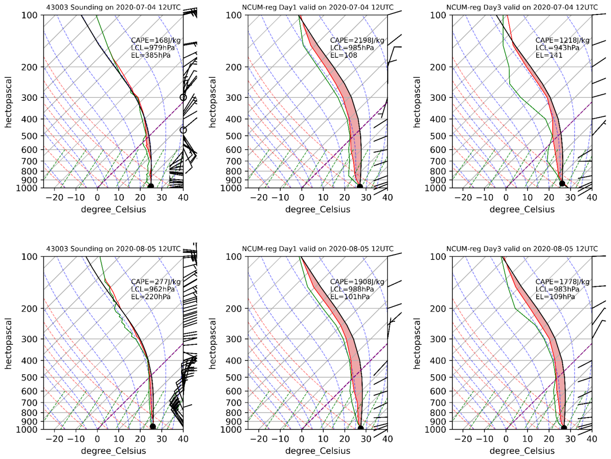
Figure S2: Same as Figure 8 but for soundings at 12 UTC
