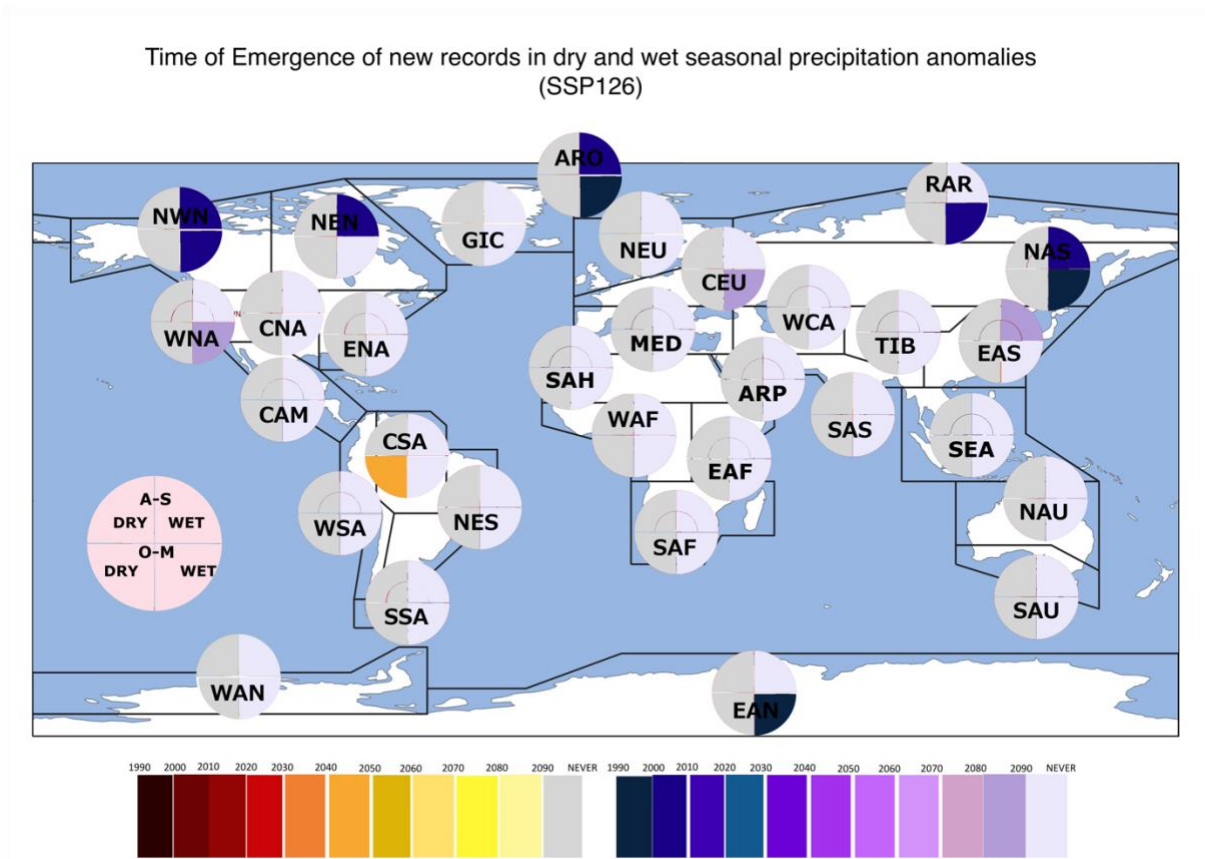
Figure S3. Time of emergence (TOE, see text for the actual definition) for all dry and wet anomaly regional cases considered, in the SSP1-2.6 scenario.
