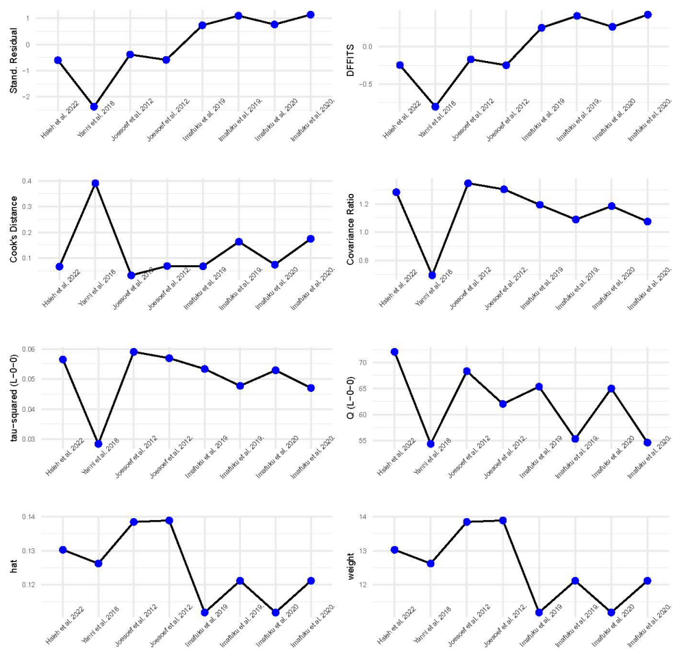
Figure 2: Influence diagnostics.
