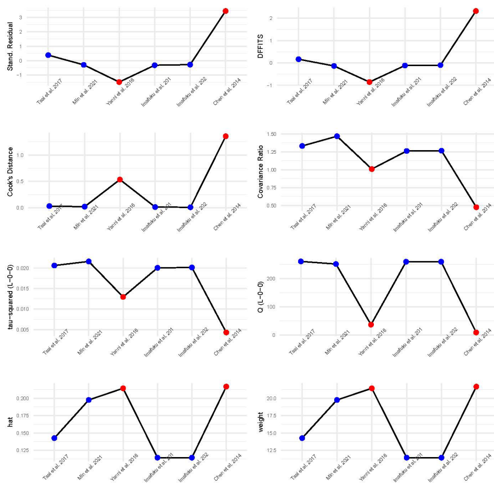
Figure 2: Influence diagnostics.
