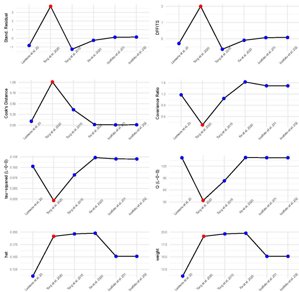
Figure 1: Baujat plot.
