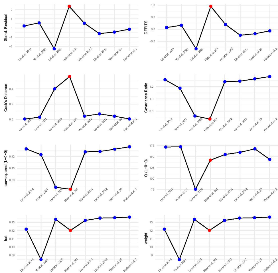
Figure 2: Influence diagnostics.
