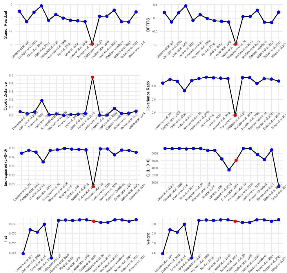
Figure 2: Influence diagnostics.
