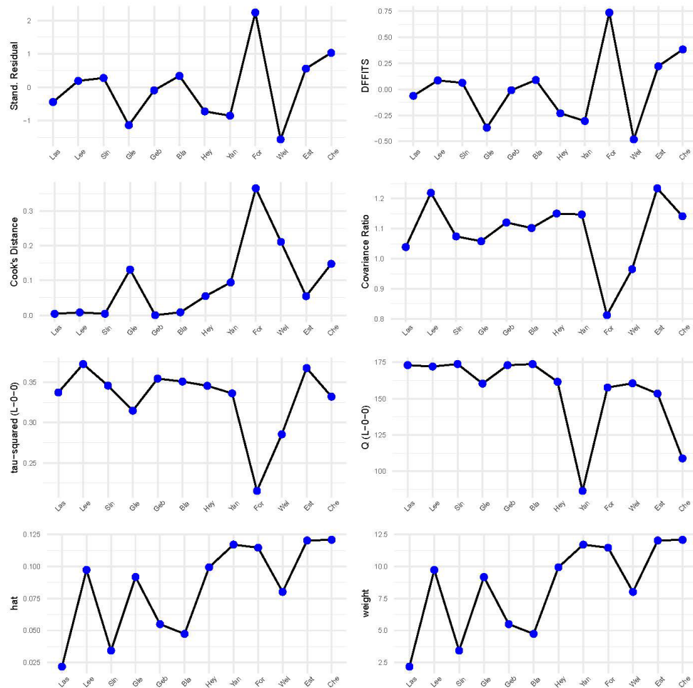
Figure 2: Influence diagnostics.
