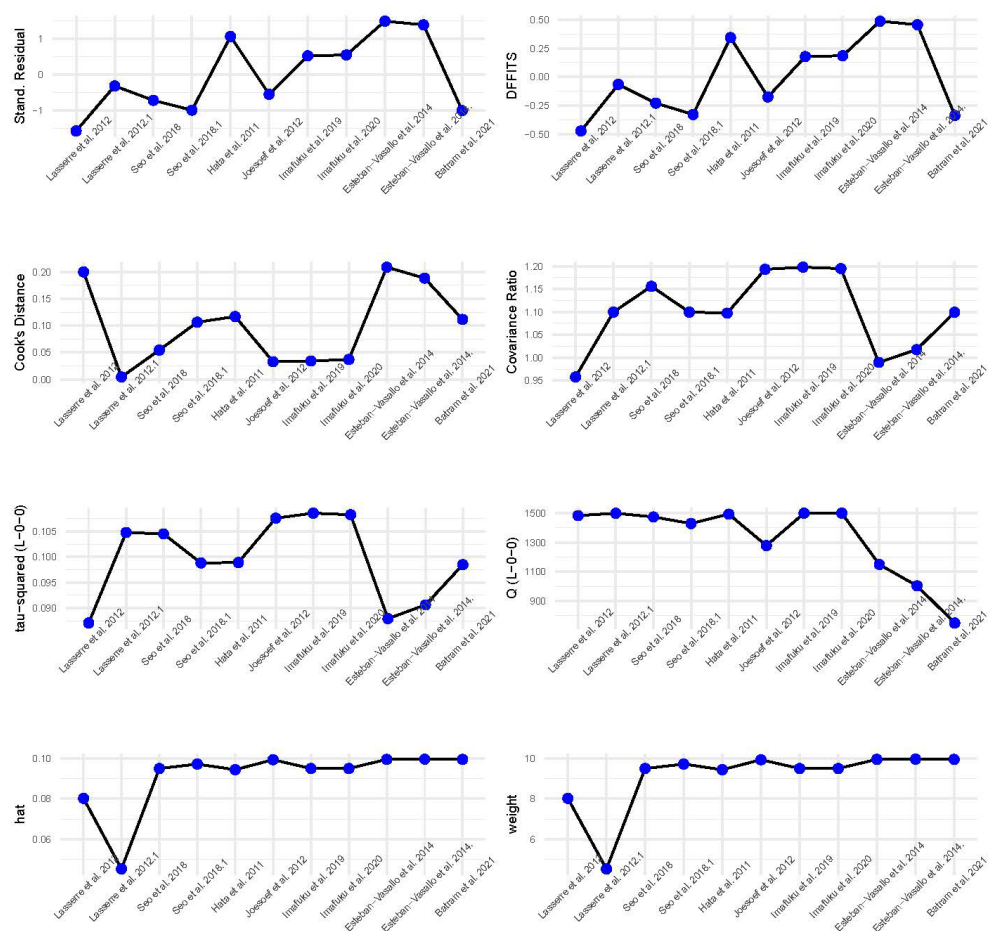
Figure 1: Baujat plot.
