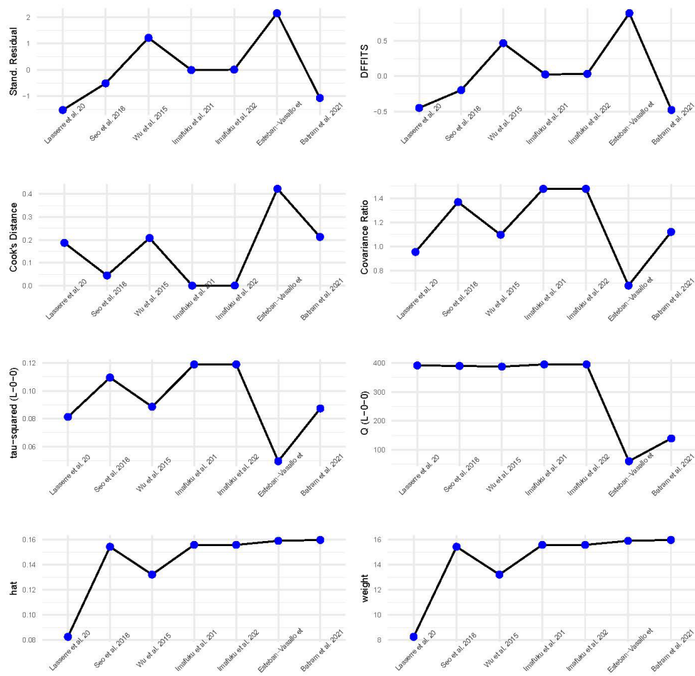
Figure 2: Influence diagnostics.
