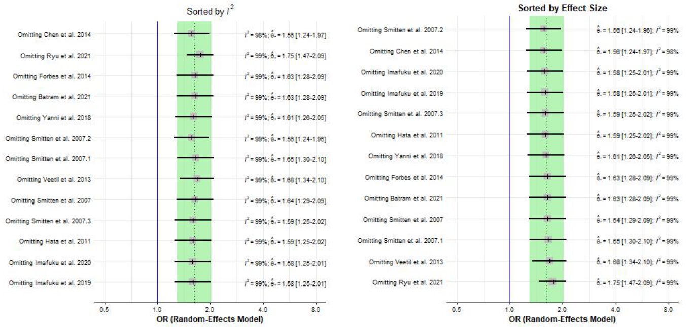
Figure 3: Forest plots for Leave-One-Out Analyses.
