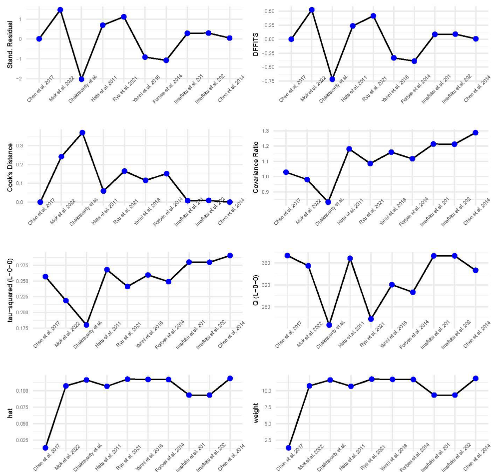
Figure 2: Influence diagnostics.
