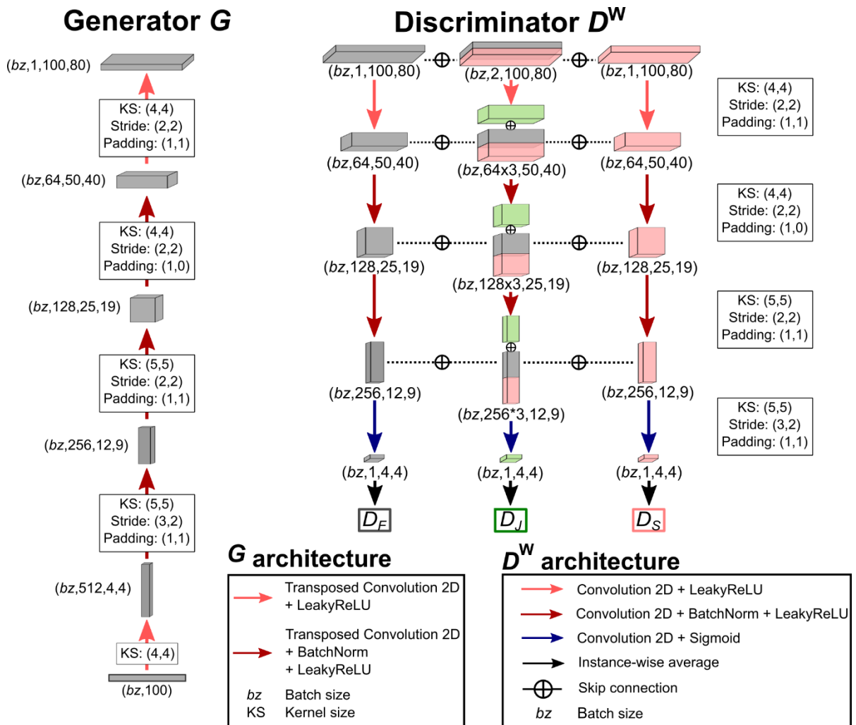
Figure S1: architecture of the W-Net GAN used for the synthetic case applications (inversion grid size 80 X 100).
