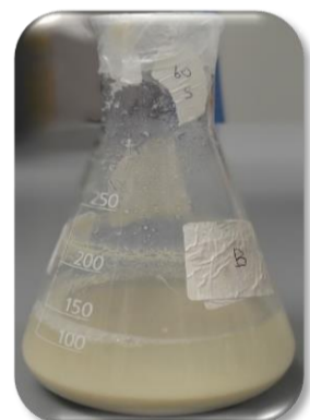
ZnO/Chitosan Nanocomposite
