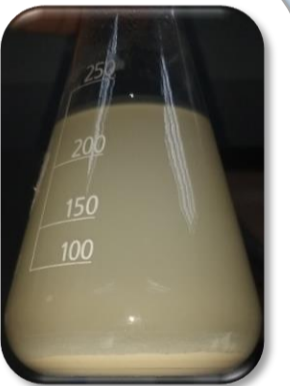
ZnO Nanoparticles
