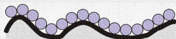
adsorbent
