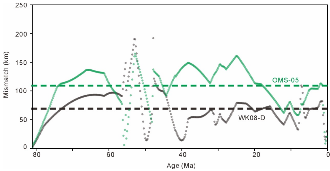
Supplementary Fig. 2. Comparison of different prediction results (based on WK-08D and OMS-05 reconstruction schemes) with coeval seamounts in the HEB. Scatters denote mismatch data, dashed lines denote average value through time.
