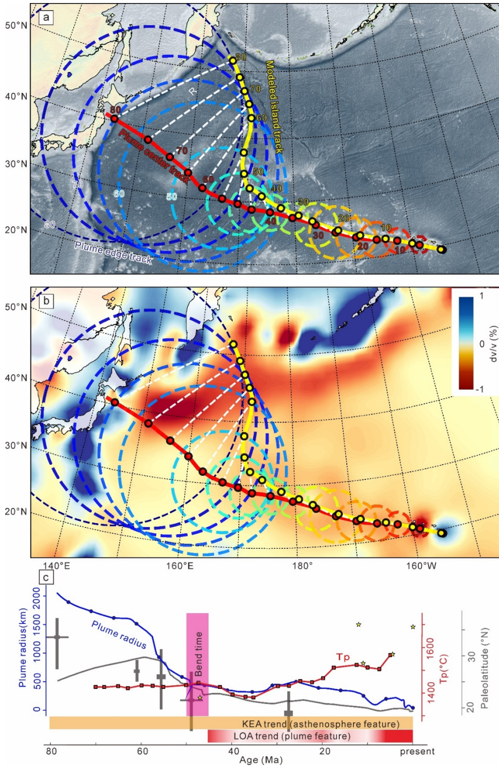
Supplementary Fig. 1. Comparison between model results (based on OMS-05 reconstruction scheme) and observation. Plume radius and predicted paleolatitude data are calculated according to the OMS-05 reconstruction scheme. Other data in c are the same as those in Figure 4c.
