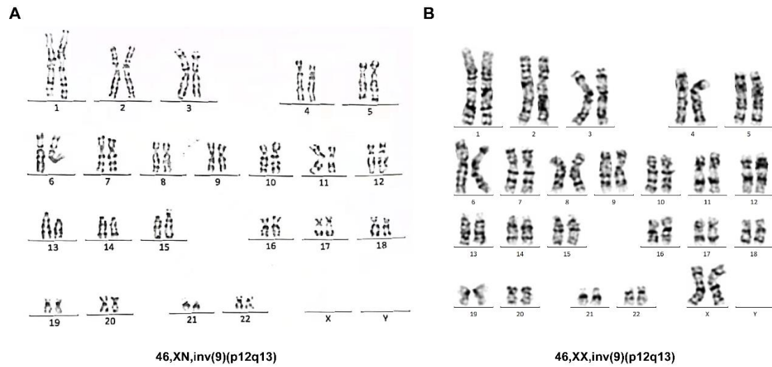
Fig. S1 Prenatal karyotype result of the fetus (A) and karyotype result of YWL. Karyotype analysis based on chromosome G-banding revealed a non-pathogenic polymorphic pericentric inversion in the fetus, 46,XN,inv(9)(p12q13), inherited from the mother (YWL).
