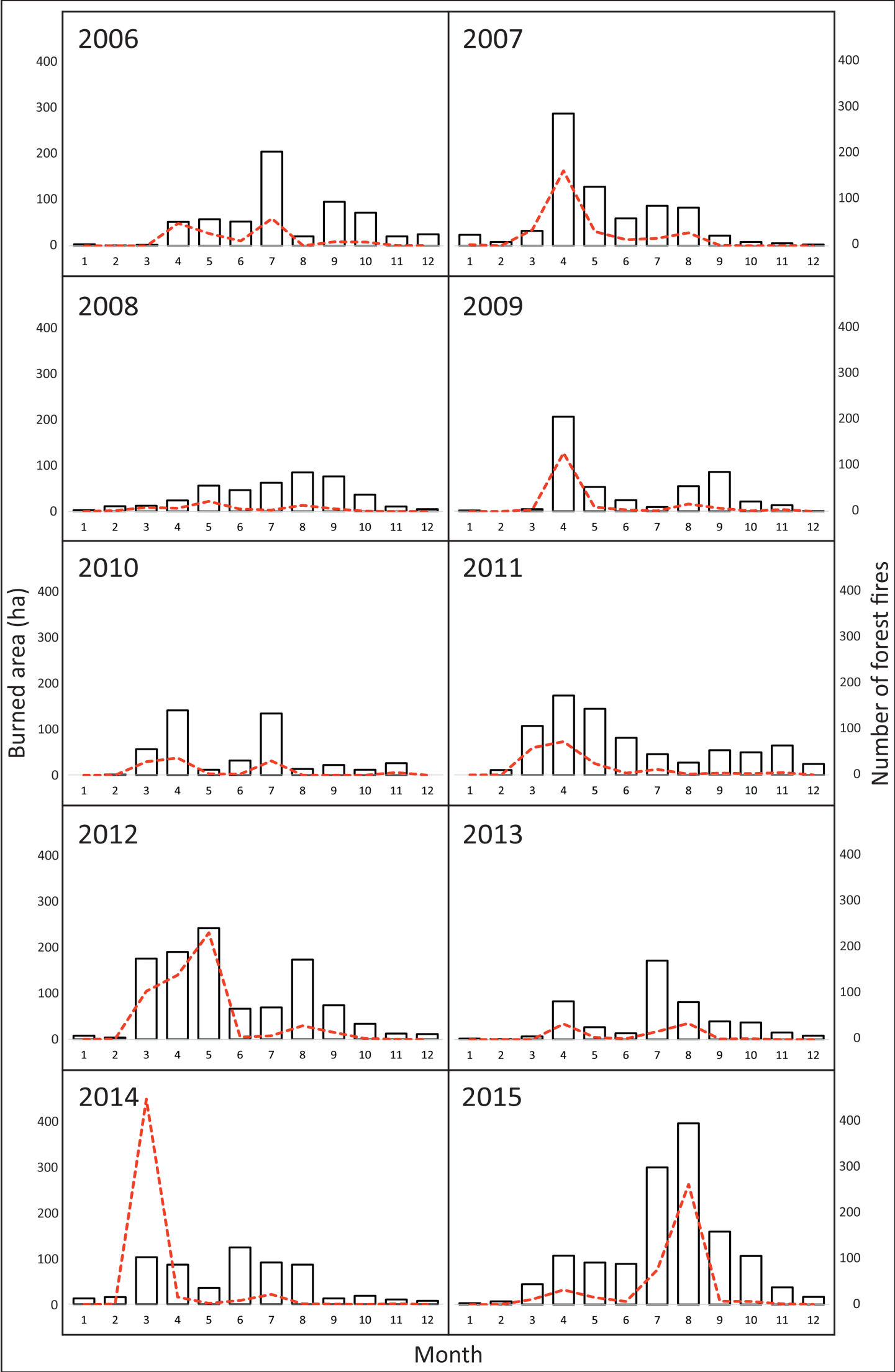
Additional file 3. Number of forest fires (bars) and burned area (red line) for each year of our study (2006 to 2015) in the Czech Republic, where we investigated the relationship between numbers of forest fires and predictor variables characterizing climate, land cover, and human activity conditions.
